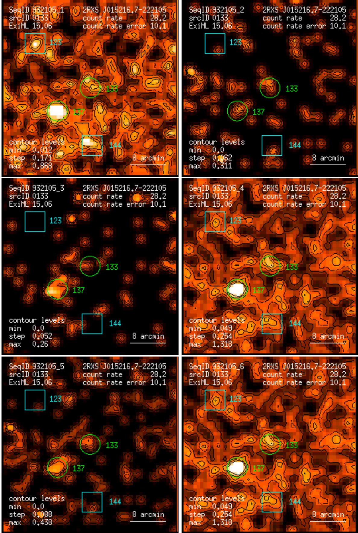
Figure 133: RASS 932105: detection 0133: band rate images, Gaussian filter: (1) PSPC channels 11 – 41, (2) 52 – 90, (3) 91 – 201, (4) 11 – 235, (5) 52 – 201, (6) 11 – 201. Broad band rates in counts/ks. Band rate contour levels in counts/ks/arcmin 2 .
