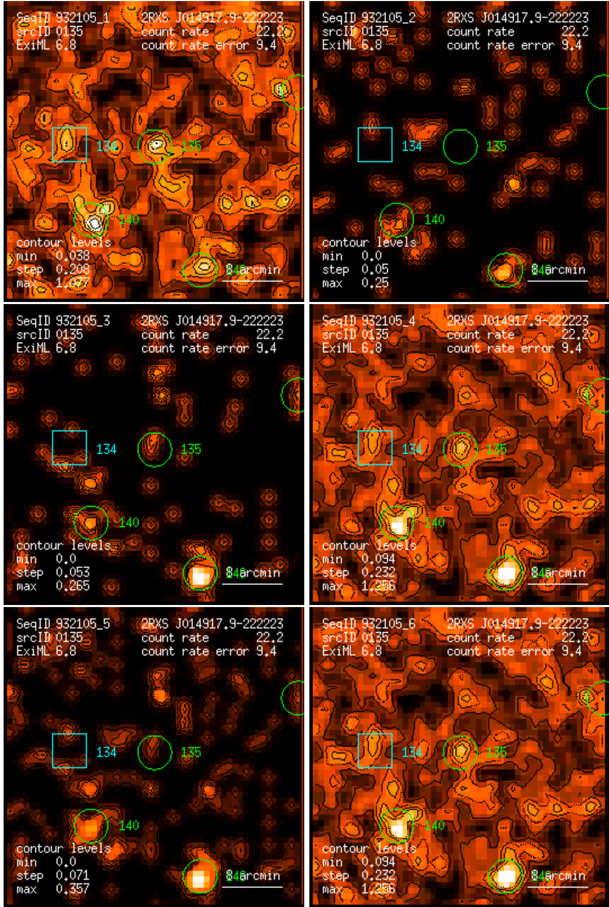
Figure 135: RASS 932105: detection 0135: band rate images, Gaussian filter: (1) PSPC channels 11 – 41, (2) 52 – 90, (3) 91 – 201, (4) 11 – 235, (5) 52 – 201, (6) 11 – 201. Broad band rates in counts/ks. Band rate contour levels in counts/ks/arcmin 2 .
