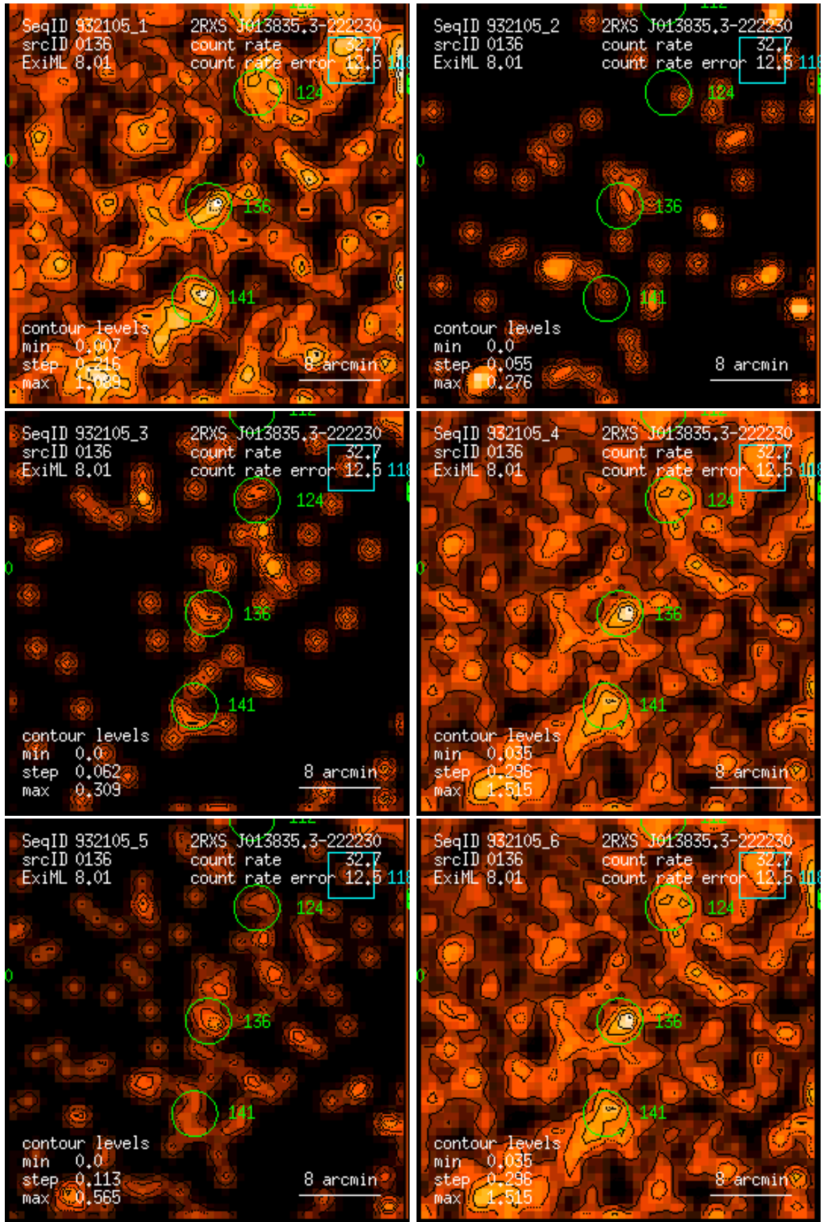
Figure 136: RASS 932105: detection 0136: band rate images, Gaussian filter: (1) PSPC channels 11 – 41, (2) 52 – 90, (3) 91 – 201, (4) 11 – 235, (5) 52 – 201, (6) 11 – 201. Broad band rates in counts/ks. Band rate contour levels in counts/ks/arcmin 2 .
