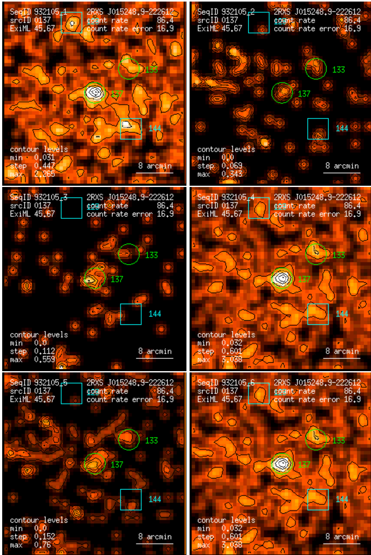
Figure 137: RASS 932105: detection 0137: band rate images, Gaussian filter: (1) PSPC channels 11 – 41, (2) 52 – 90, (3) 91 – 201, (4) 11 – 235, (5) 52 – 201, (6) 11 – 201. Broad band rates in counts/ks. Band rate contour levels in counts/ks/arcmin 2 .
