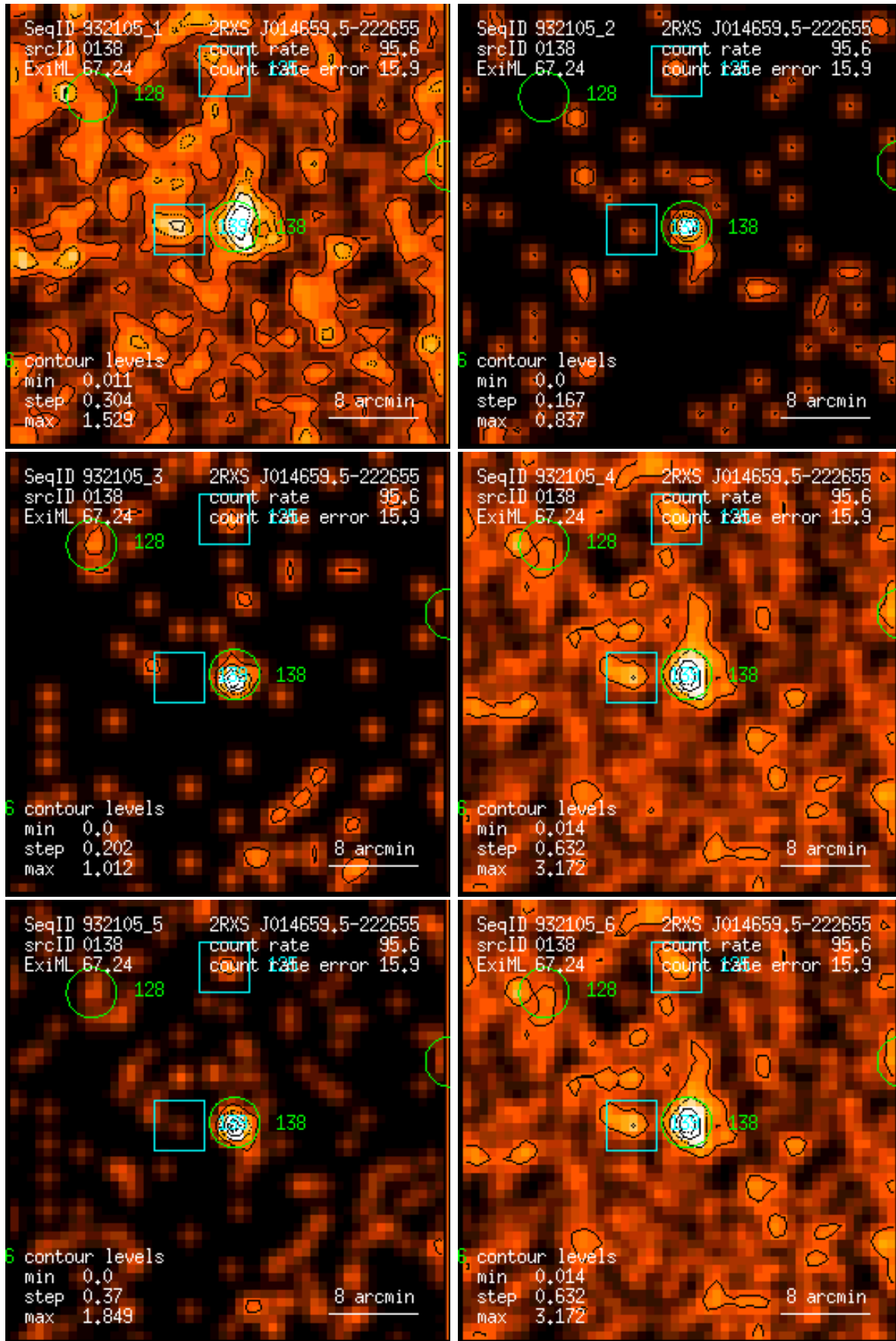
Figure 138: RASS 932105: detection 0138: band rate images, Gaussian filter: (1) PSPC channels 11 – 41, (2) 52 – 90, (3) 91 – 201, (4) 11 – 235, (5) 52 – 201, (6) 11 – 201. Broad band rates in counts/ks. Band rate contour levels in counts/ks/arcmin 2 .
