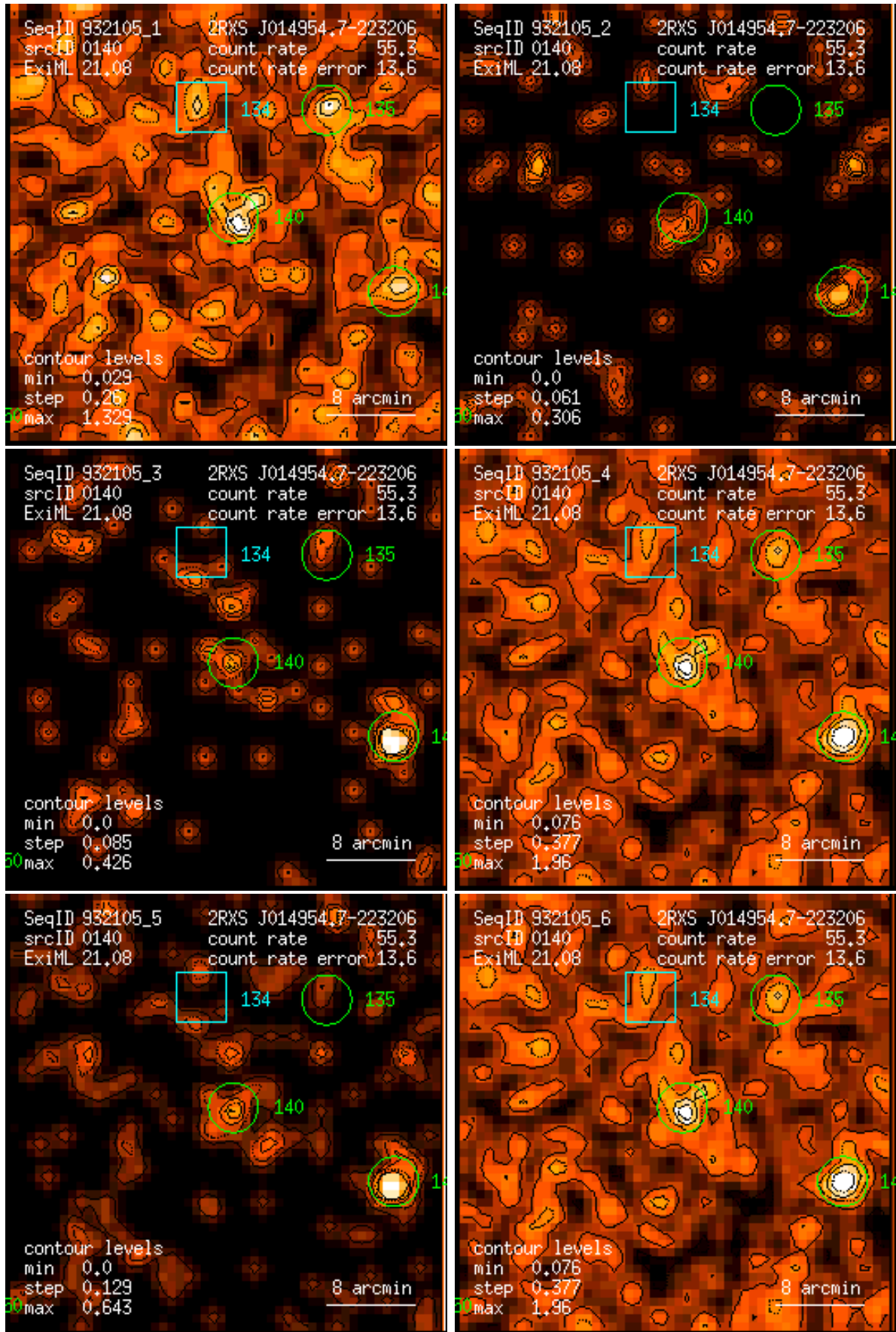
Figure 140: RASS 932105: detection 0140: band rate images, Gaussian filter: (1) PSPC channels 11 – 41, (2) 52 – 90, (3) 91 – 201, (4) 11 – 235, (5) 52 – 201, (6) 11 – 201. Broad band rates in counts/ks. Band rate contour levels in counts/ks/arcmin 2 .
