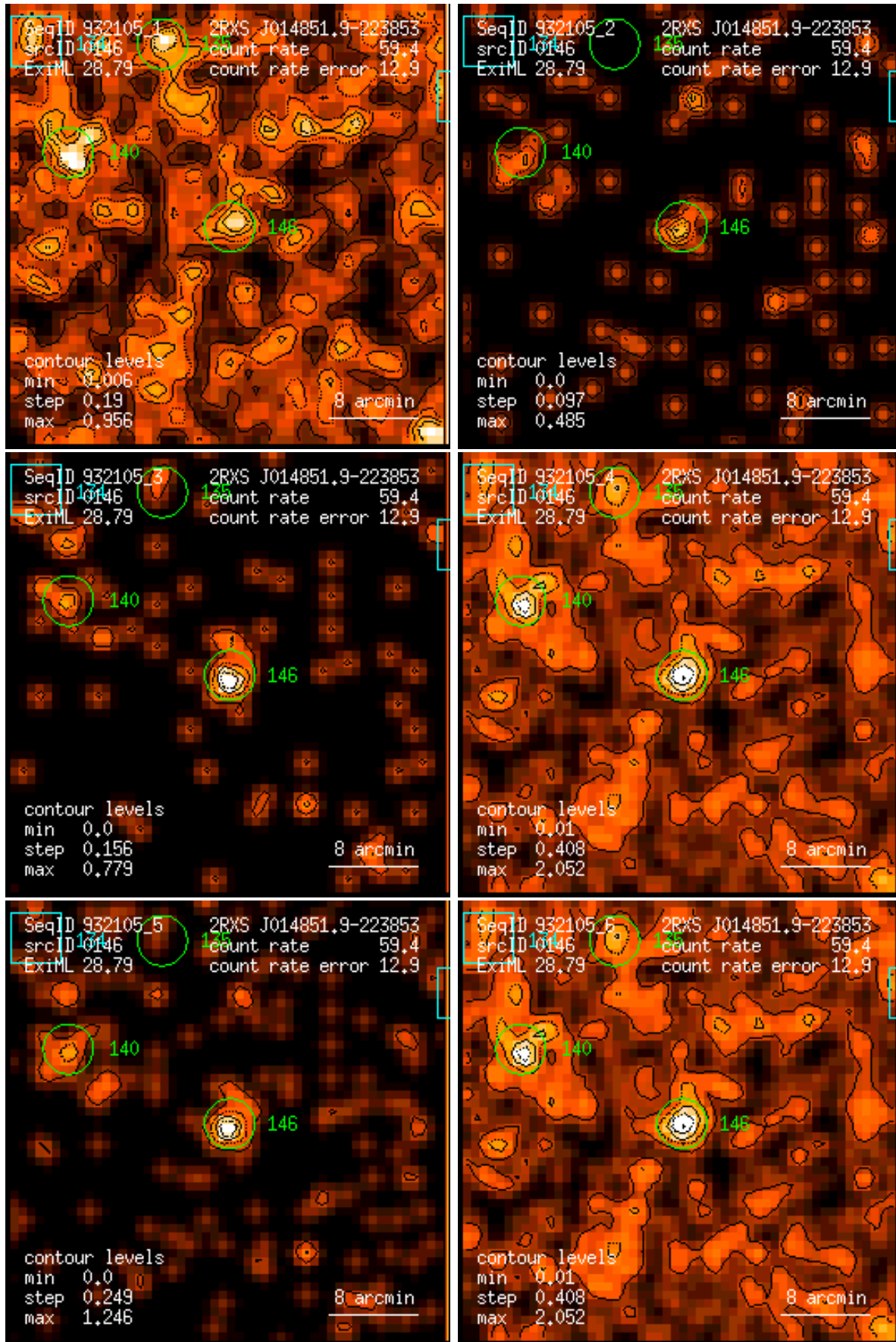
Figure 146: RASS 932105: detection 0146: band rate images, Gaussian filter: (1) PSPC channels 11 – 41, (2) 52 – 90, (3) 91 – 201, (4) 11 – 235, (5) 52 – 201, (6) 11 – 201. Broad band rates in counts/ks. Band rate contour levels in counts/ks/arcmin 2 .
