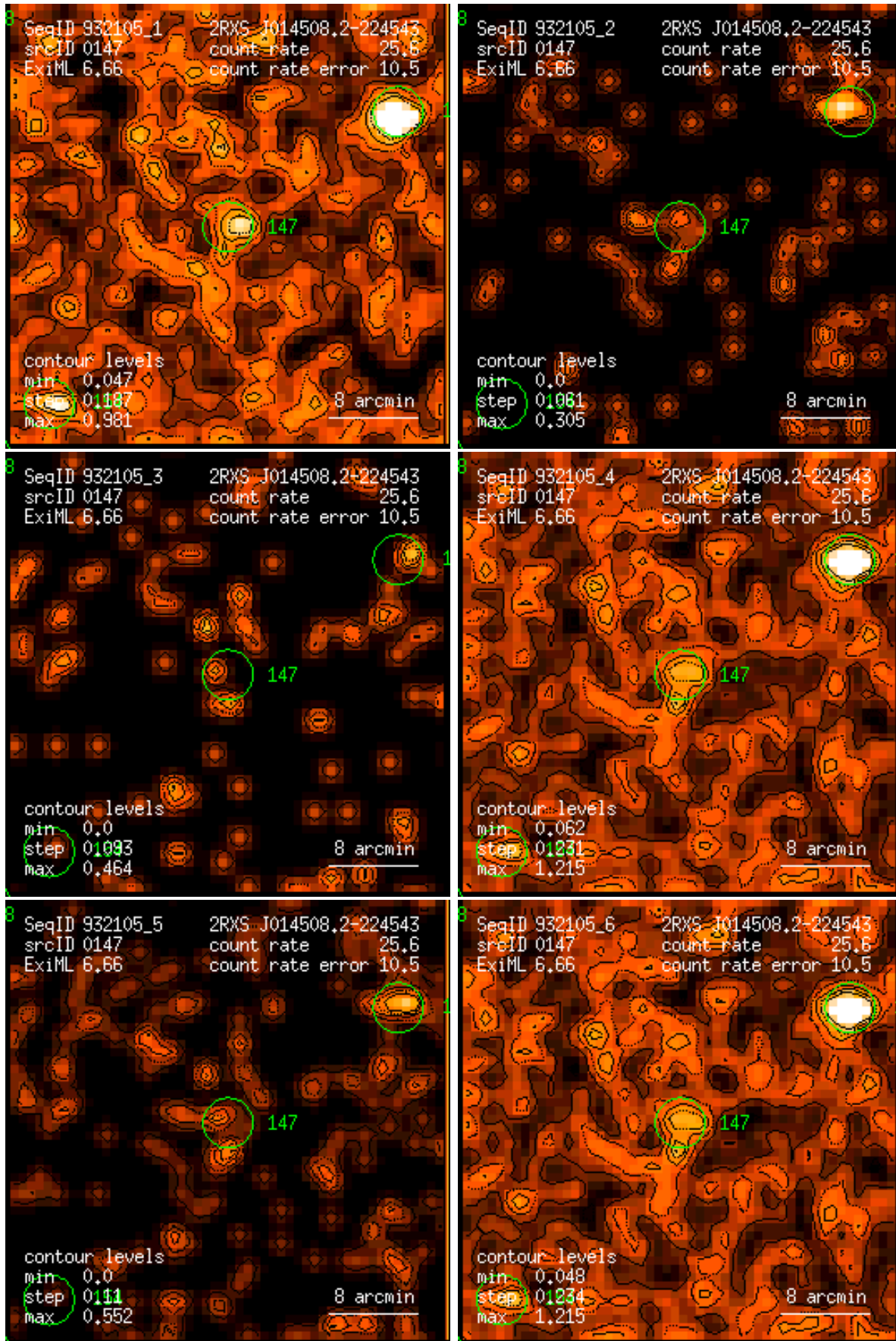
Figure 147: RASS 932105: detection 0147: band rate images, Gaussian filter: (1) PSPC channels 11 – 41, (2) 52 – 90, (3) 91 – 201, (4) 11 – 235, (5) 52 – 201, (6) 11 – 201. Broad band rates in counts/ks. Band rate contour levels in counts/ks/arcmin 2 .
