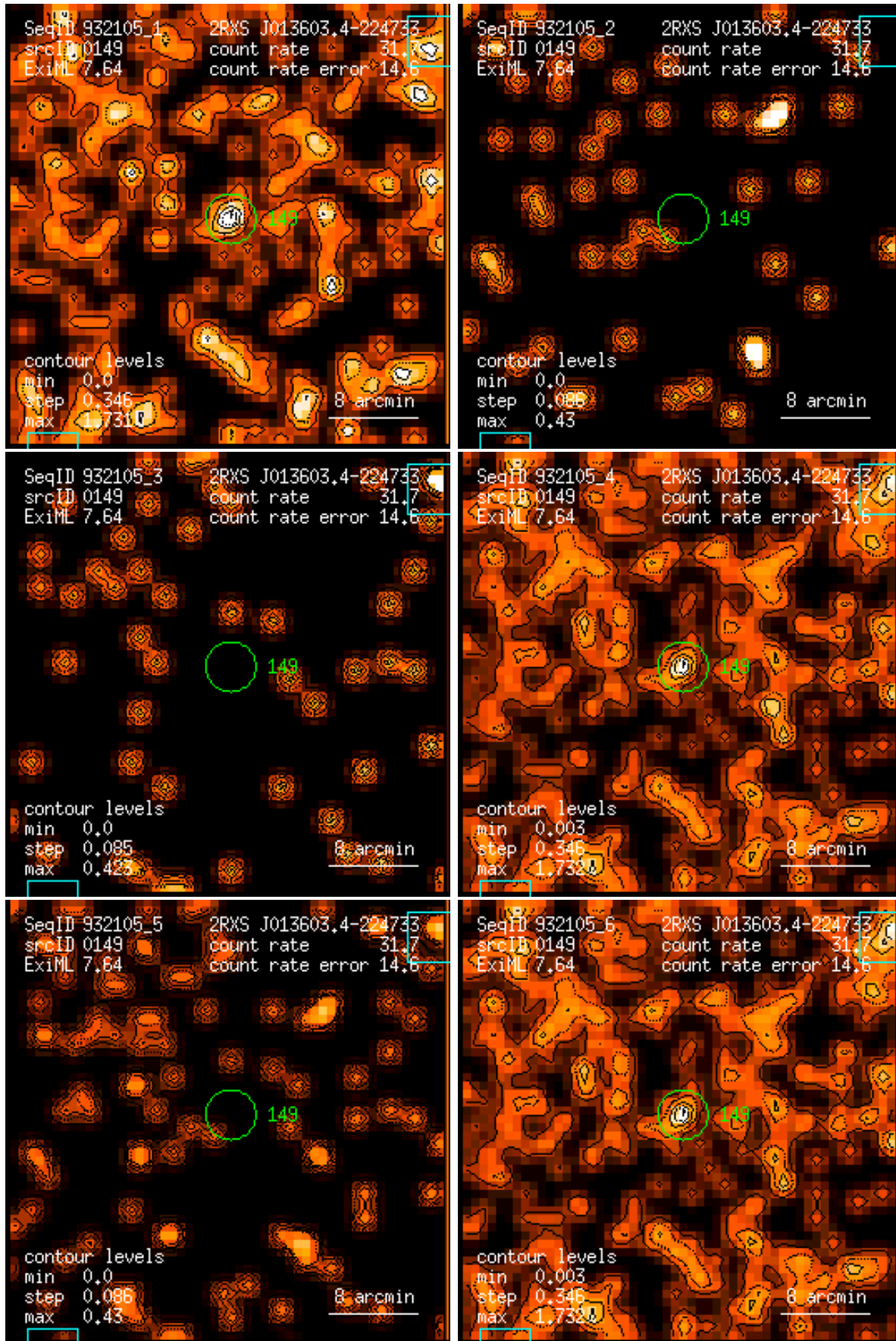
Figure 149: RASS 932105: detection 0149: band rate images, Gaussian filter: (1) PSPC channels 11 – 41, (2) 52 – 90, (3) 91 – 201, (4) 11 – 235, (5) 52 – 201, (6) 11 – 201. Broad band rates in counts/ks. Band rate contour levels in counts/ks/arcmin 2 .
