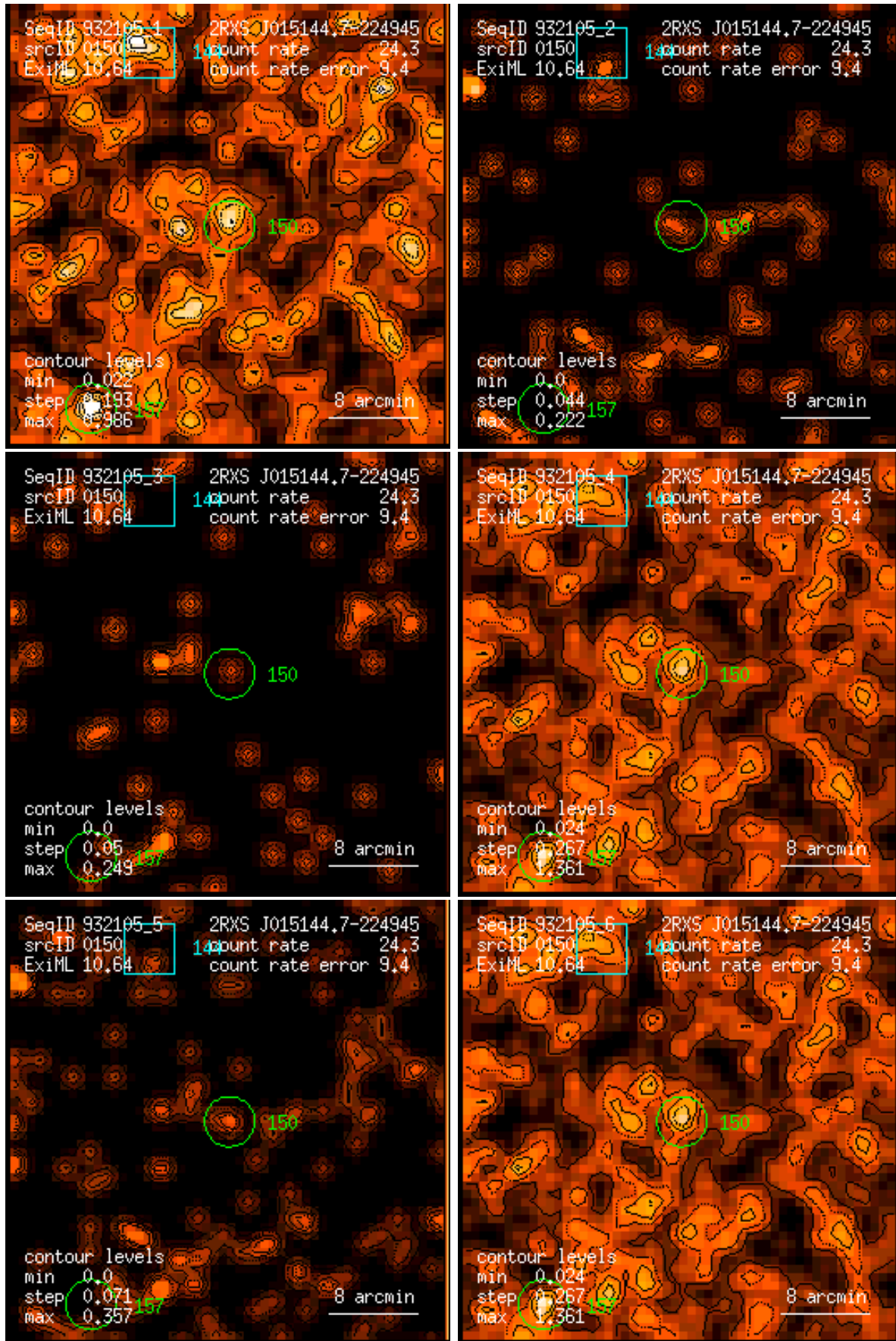
Figure 150: RASS 932105: detection 0150: band rate images, Gaussian filter: (1) PSPC channels 11 – 41, (2) 52 – 90, (3) 91 – 201, (4) 11 – 235, (5) 52 – 201, (6) 11 – 201. Broad band rates in counts/ks. Band rate contour levels in counts/ks/arcmin 2 .
