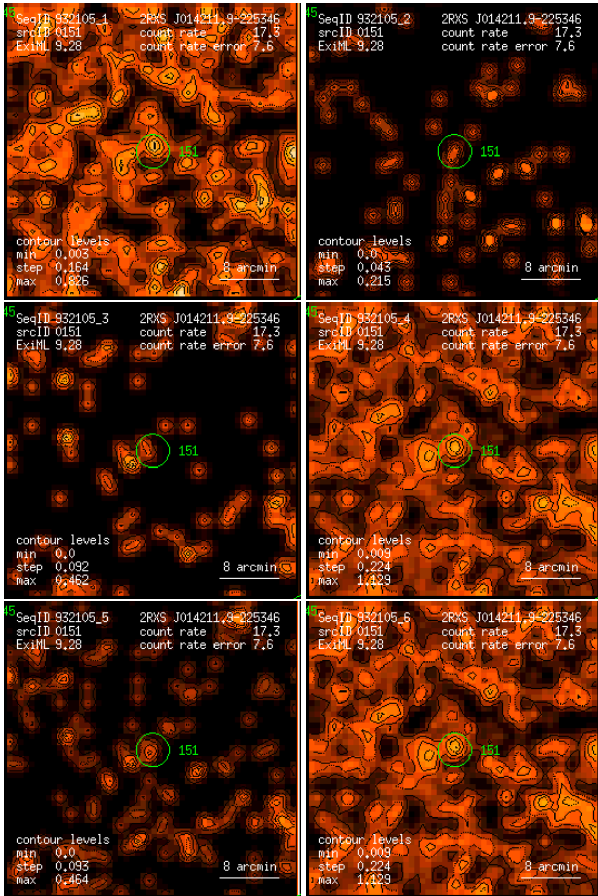
Figure 151: RASS 932105: detection 0151: band rate images, Gaussian filter: (1) PSPC channels 11 – 41, (2) 52 – 90, (3) 91 – 201, (4) 11 – 235, (5) 52 – 201, (6) 11 – 201. Broad band rates in counts/ks. Band rate contour levels in counts/ks/arcmin 2 .
