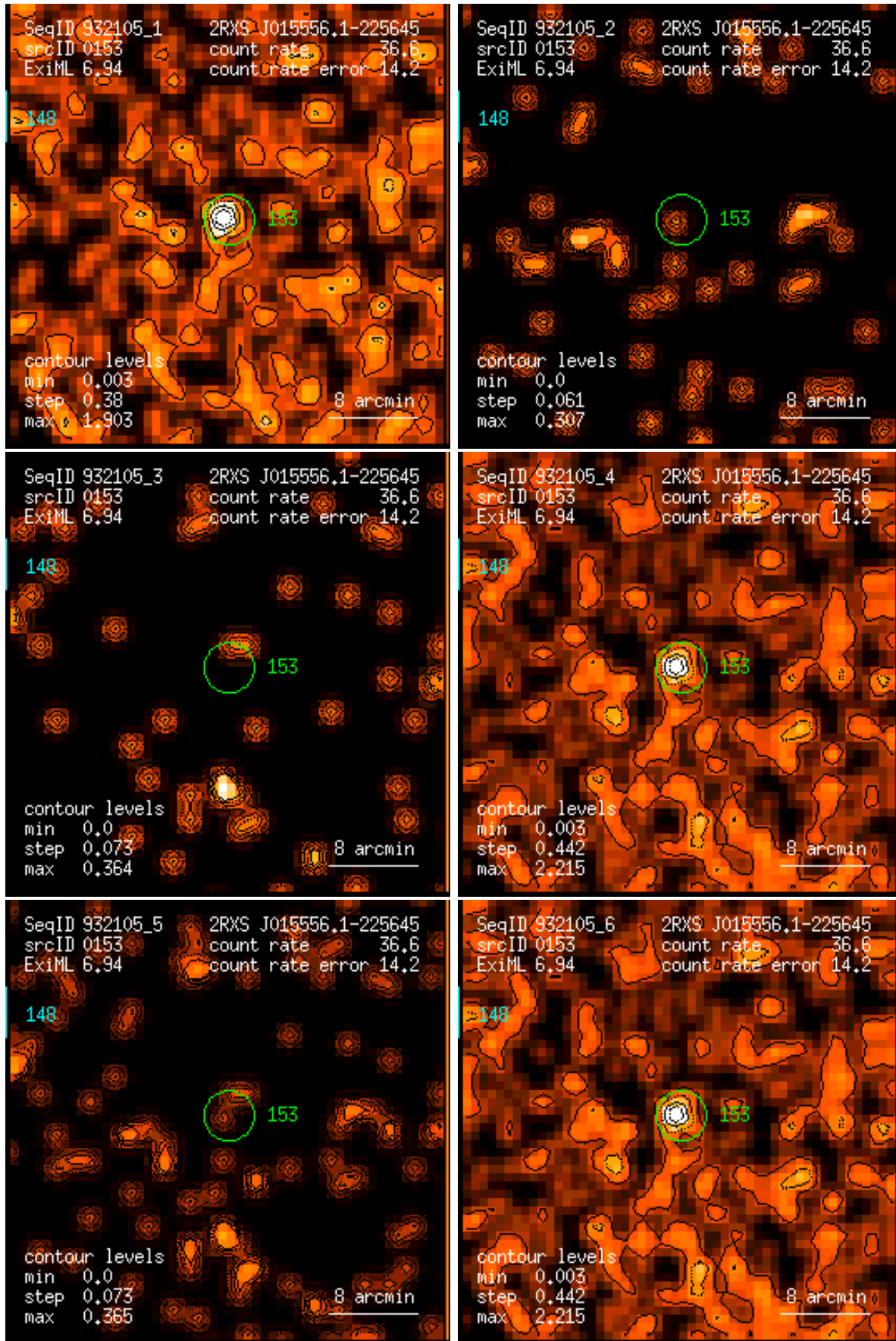
Figure 153: RASS 932105: detection 0153: band rate images, Gaussian filter: (1) PSPC channels 11 – 41, (2) 52 – 90, (3) 91 – 201, (4) 11 – 235, (5) 52 – 201, (6) 11 – 201. Broad band rates in counts/ks. Band rate contour levels in counts/ks/arcmin 2 .
