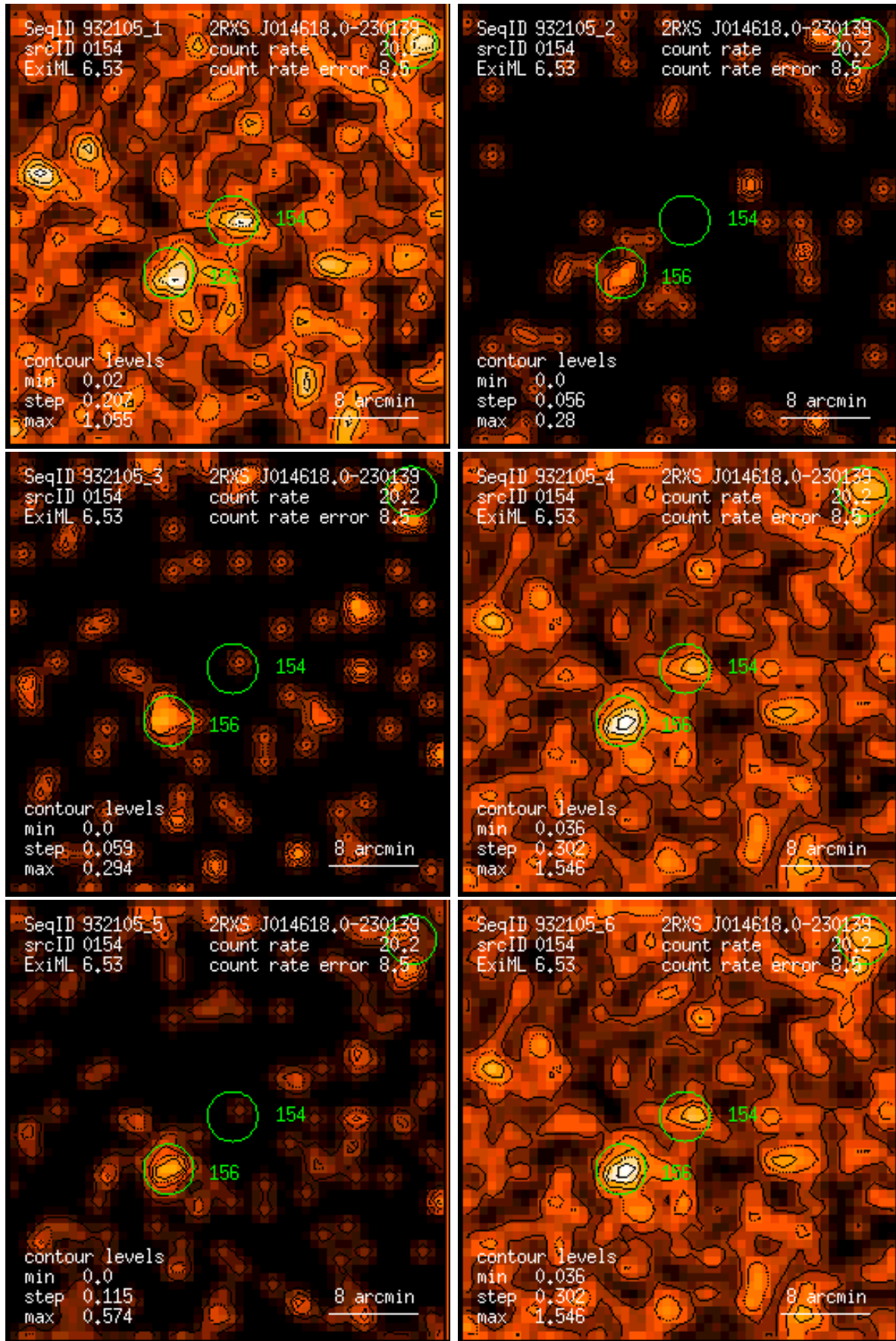
Figure 154: RASS 932105: detection 0154: band rate images, Gaussian filter: (1) PSPC channels 11 – 41, (2) 52 – 90, (3) 91 – 201, (4) 11 – 235, (5) 52 – 201, (6) 11 – 201. Broad band rates in counts/ks. Band rate contour levels in counts/ks/arcmin 2 .
