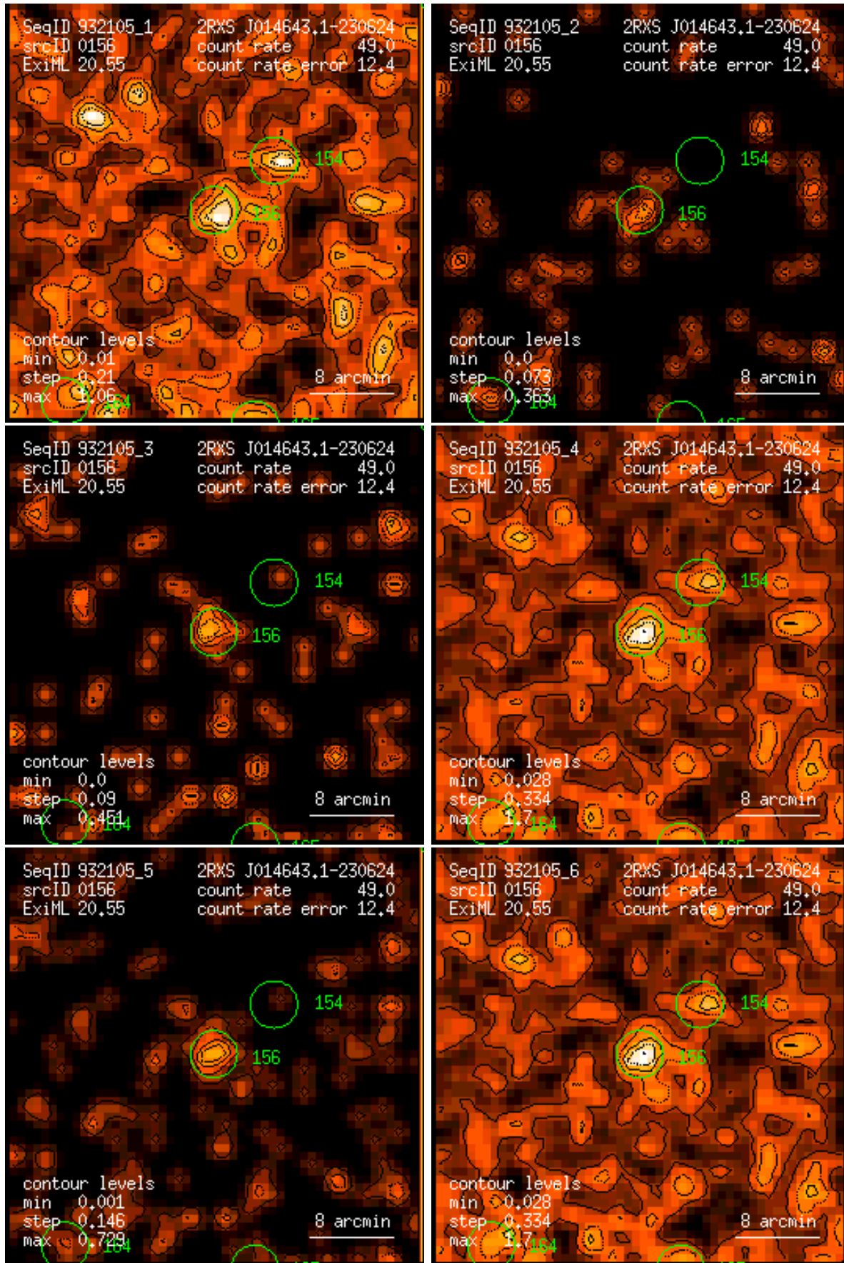
Figure 156: RASS 932105: detection 0156: band rate images, Gaussian filter: (1) PSPC channels 11 – 41, (2) 52 – 90, (3) 91 – 201, (4) 11 – 235, (5) 52 – 201, (6) 11 – 201. Broad band rates in counts/ks. Band rate contour levels in counts/ks/arcmin 2 .
