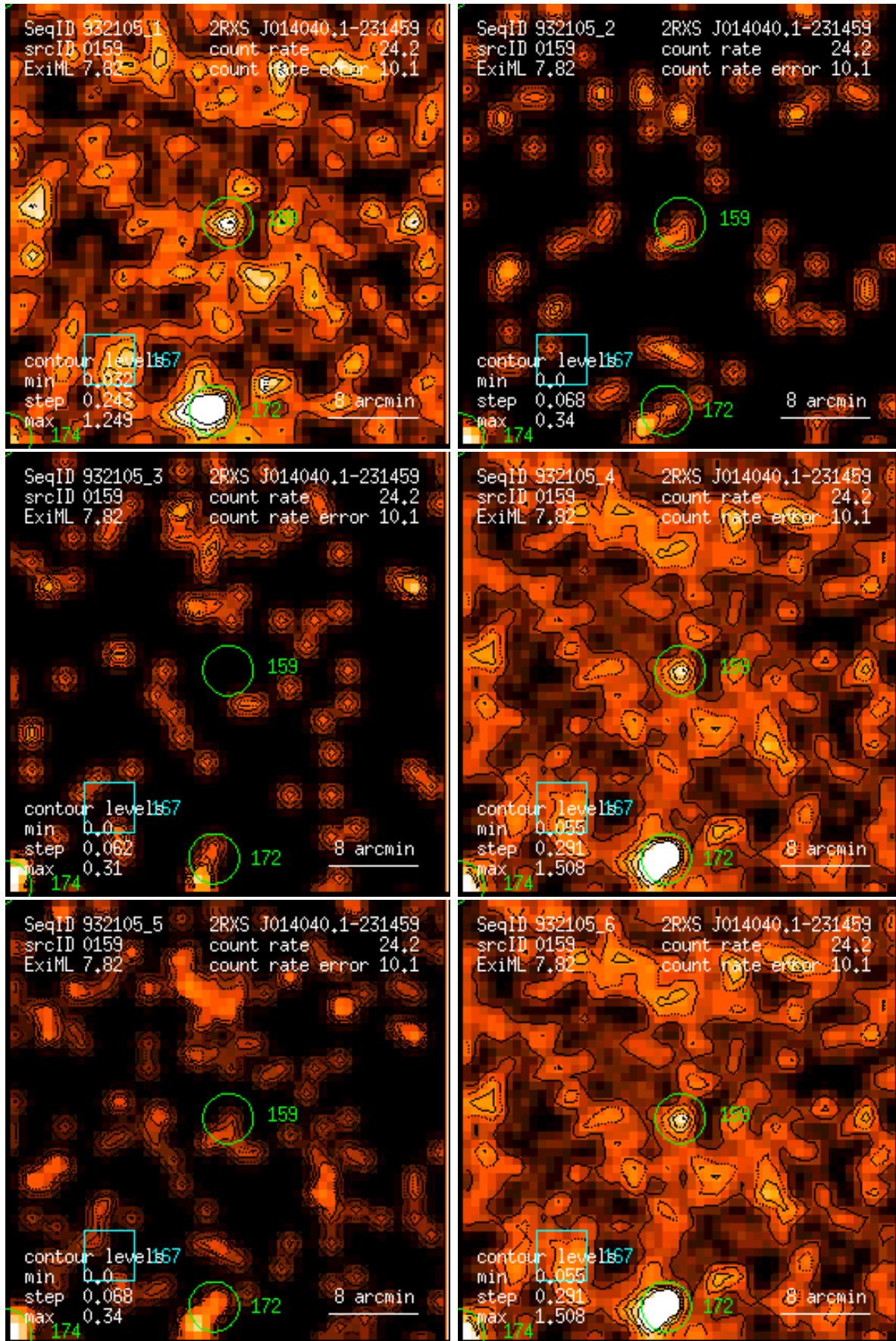
Figure 159: RASS 932105: detection 0159: band rate images, Gaussian filter: (1) PSPC channels 11 – 41, (2) 52 – 90, (3) 91 – 201, (4) 11 – 235, (5) 52 – 201, (6) 11 – 201. Broad band rates in counts/ks. Band rate contour levels in counts/ks/arcmin 2 .
