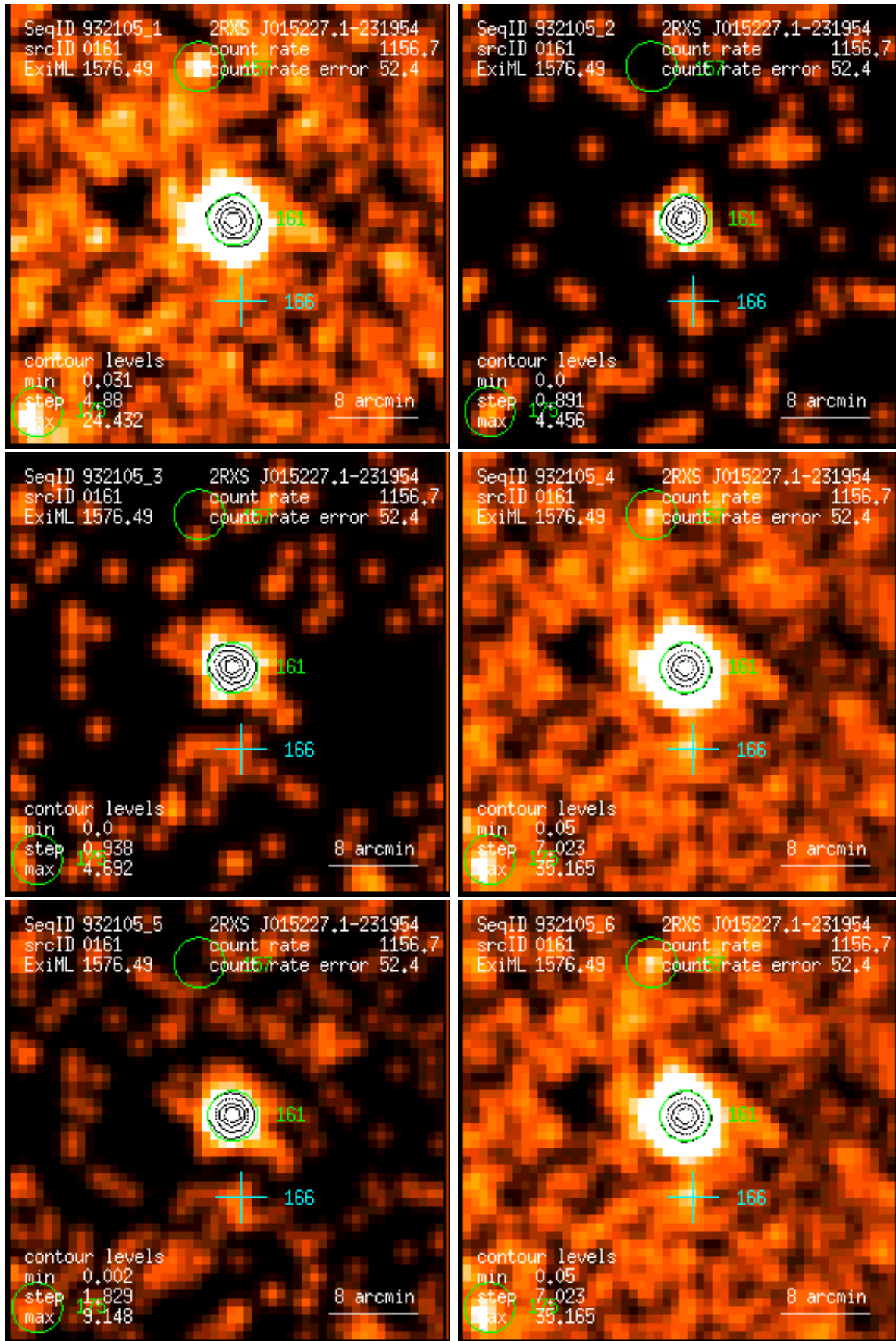
Figure 161: RASS 932105: detection 0161: band rate images, Gaussian filter: (1) PSPC channels 11 – 41, (2) 52 – 90, (3) 91 – 201, (4) 11 – 235, (5) 52 – 201, (6) 11 – 201. Broad band rates in counts/ks. Band rate contour levels in counts/ks/arcmin 2 .
