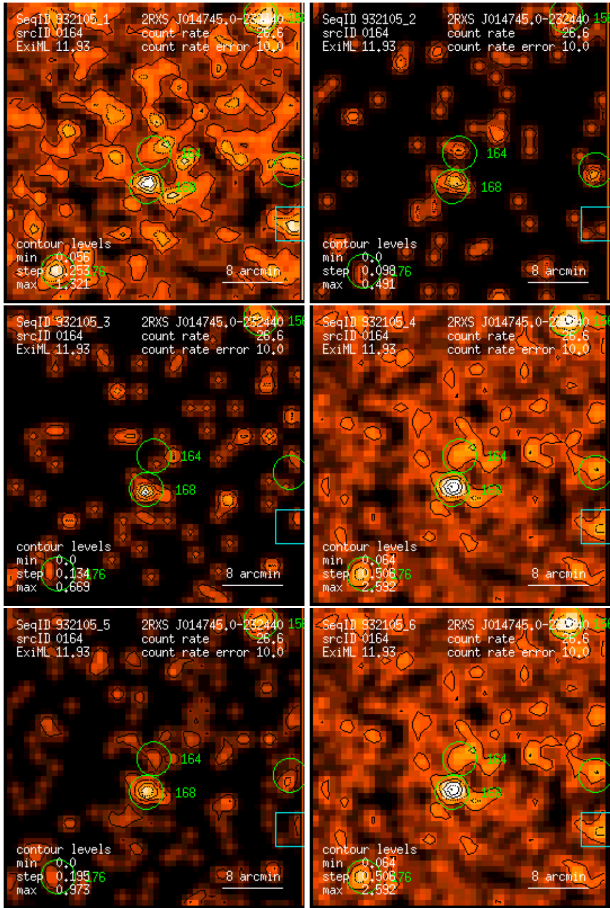
Figure 164: RASS 932105: detection 0164: band rate images, Gaussian filter: (1) PSPC channels 11 – 41, (2) 52 – 90, (3) 91 – 201, (4) 11 – 235, (5) 52 – 201, (6) 11 – 201. Broad band rates in counts/ks. Band rate contour levels in counts/ks/arcmin 2 .
