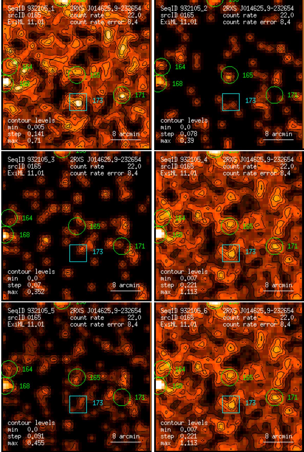
Figure 165: RASS 932105: detection 0165: band rate images, Gaussian filter: (1) PSPC channels 11 – 41, (2) 52 – 90, (3) 91 – 201, (4) 11 – 235, (5) 52 – 201, (6) 11 – 201. Broad band rates in counts/ks. Band rate contour levels in counts/ks/arcmin 2 .
