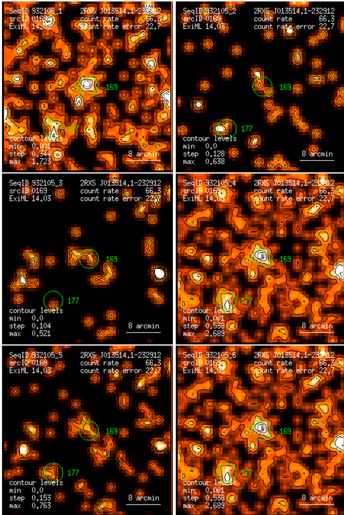
Figure 169: RASS 932105: detection 0169: band rate images, Gaussian filter: (1) PSPC channels 11 – 41, (2) 52 – 90, (3) 91 – 201, (4) 11 – 235, (5) 52 – 201, (6) 11 – 201. Broad band rates in counts/ks. Band rate contour levels in counts/ks/arcmin 2 .
