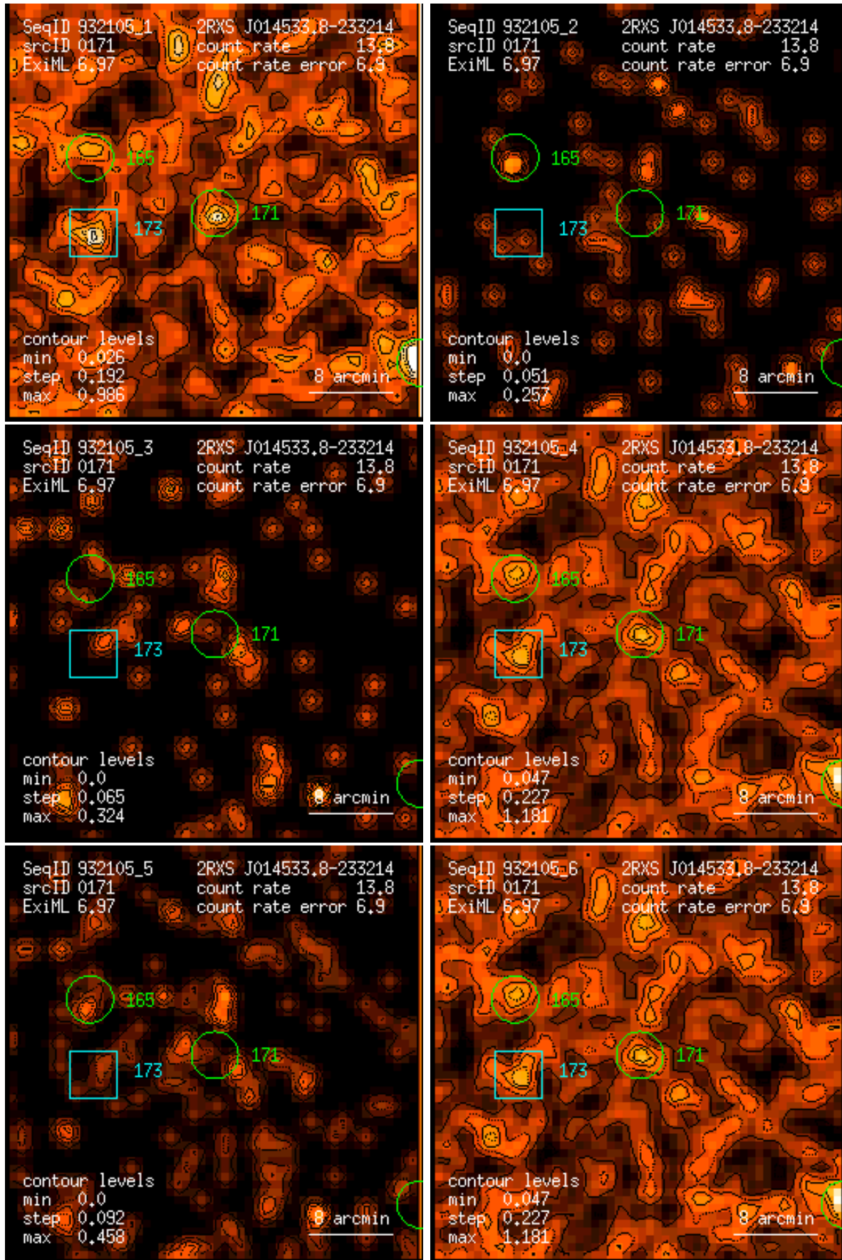
Figure 171: RASS 932105: detection 0171: band rate images, Gaussian filter: (1) PSPC channels 11 – 41, (2) 52 – 90, (3) 91 – 201, (4) 11 – 235, (5) 52 – 201, (6) 11 – 201. Broad band rates in counts/ks. Band rate contour levels in counts/ks/arcmin 2 .
