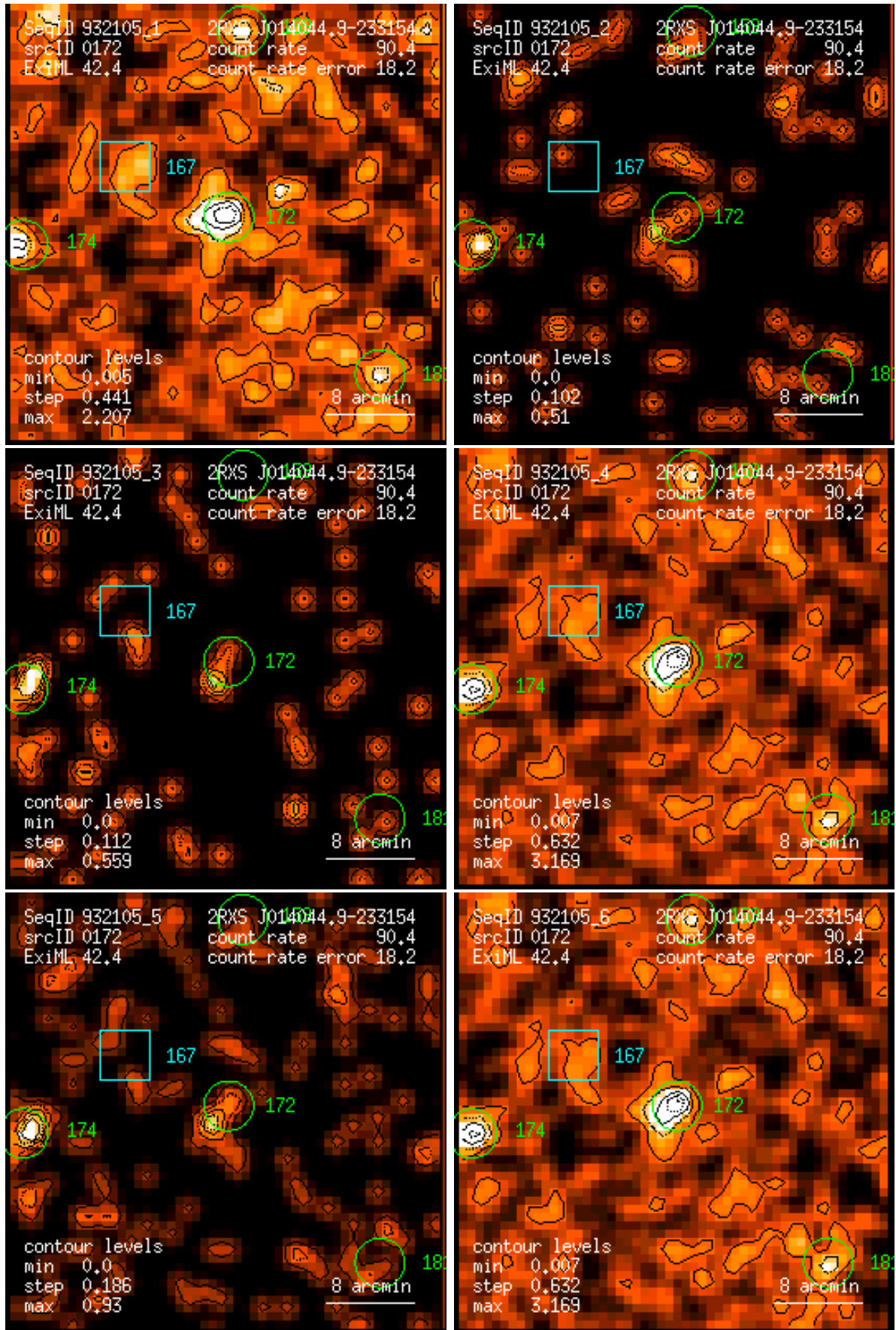
Figure 172: RASS 932105: detection 0172: band rate images, Gaussian filter: (1) PSPC channels 11 – 41, (2) 52 – 90, (3) 91 – 201, (4) 11 – 235, (5) 52 – 201, (6) 11 – 201. Broad band rates in counts/ks. Band rate contour levels in counts/ks/arcmin 2 .
