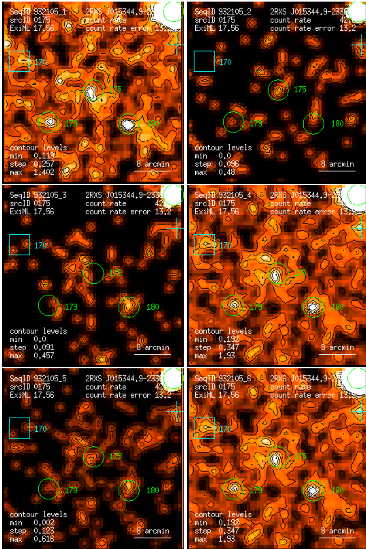
Figure 175: RASS 932105: detection 0175: band rate images, Gaussian filter: (1) PSPC channels 11 – 41, (2) 52 – 90, (3) 91 – 201, (4) 11 – 235, (5) 52 – 201, (6) 11 – 201. Broad band rates in counts/ks. Band rate contour levels in counts/ks/arcmin 2 .
