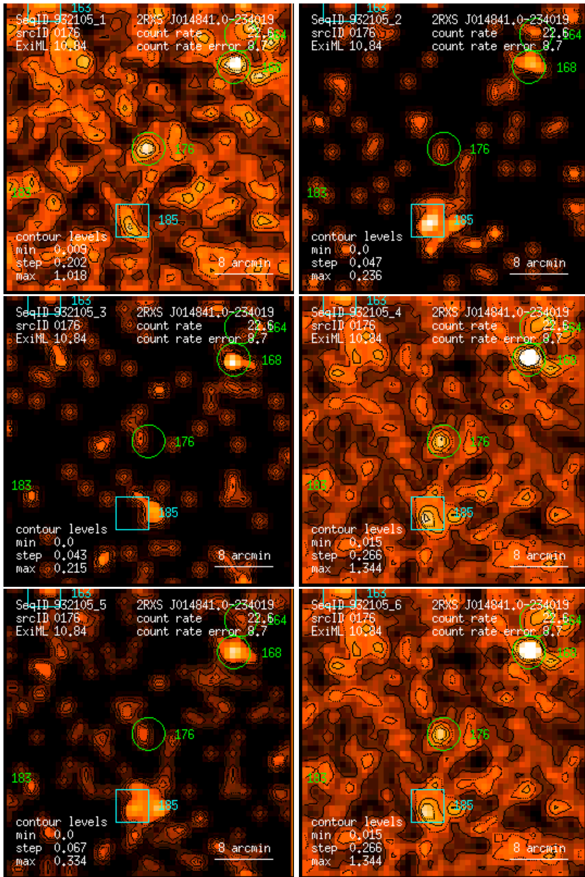
Figure 176: RASS 932105: detection 0176: band rate images, Gaussian filter: (1) PSPC channels 11 – 41, (2) 52 – 90, (3) 91 – 201, (4) 11 – 235, (5) 52 – 201, (6) 11 – 201. Broad band rates in counts/ks. Band rate contour levels in counts/ks/arcmin 2 .
