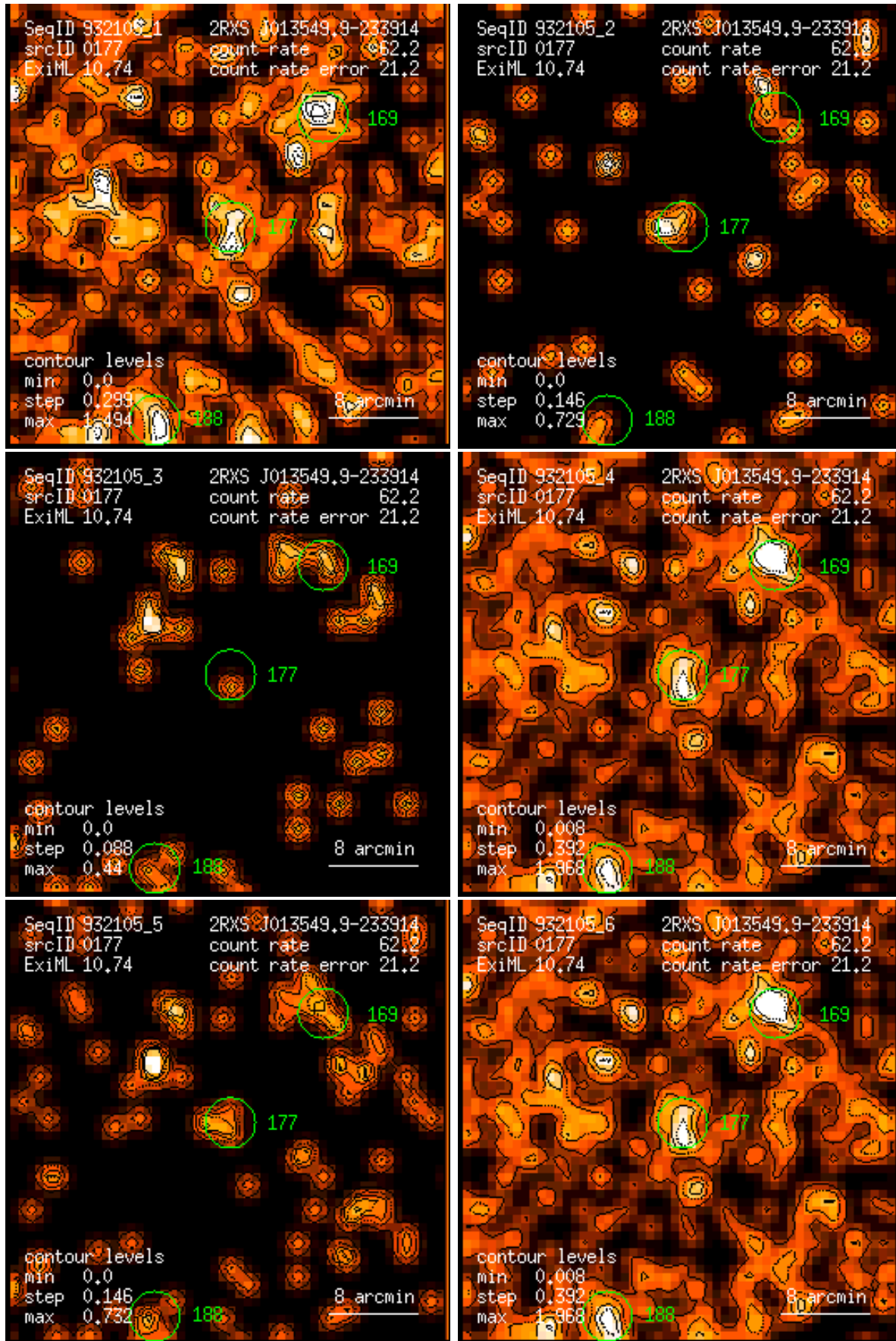
Figure 177: RASS 932105: detection 0177: band rate images, Gaussian filter: (1) PSPC channels 11 – 41, (2) 52 – 90, (3) 91 – 201, (4) 11 – 235, (5) 52 – 201, (6) 11 – 201. Broad band rates in counts/ks. Band rate contour levels in counts/ks/arcmin 2 .
