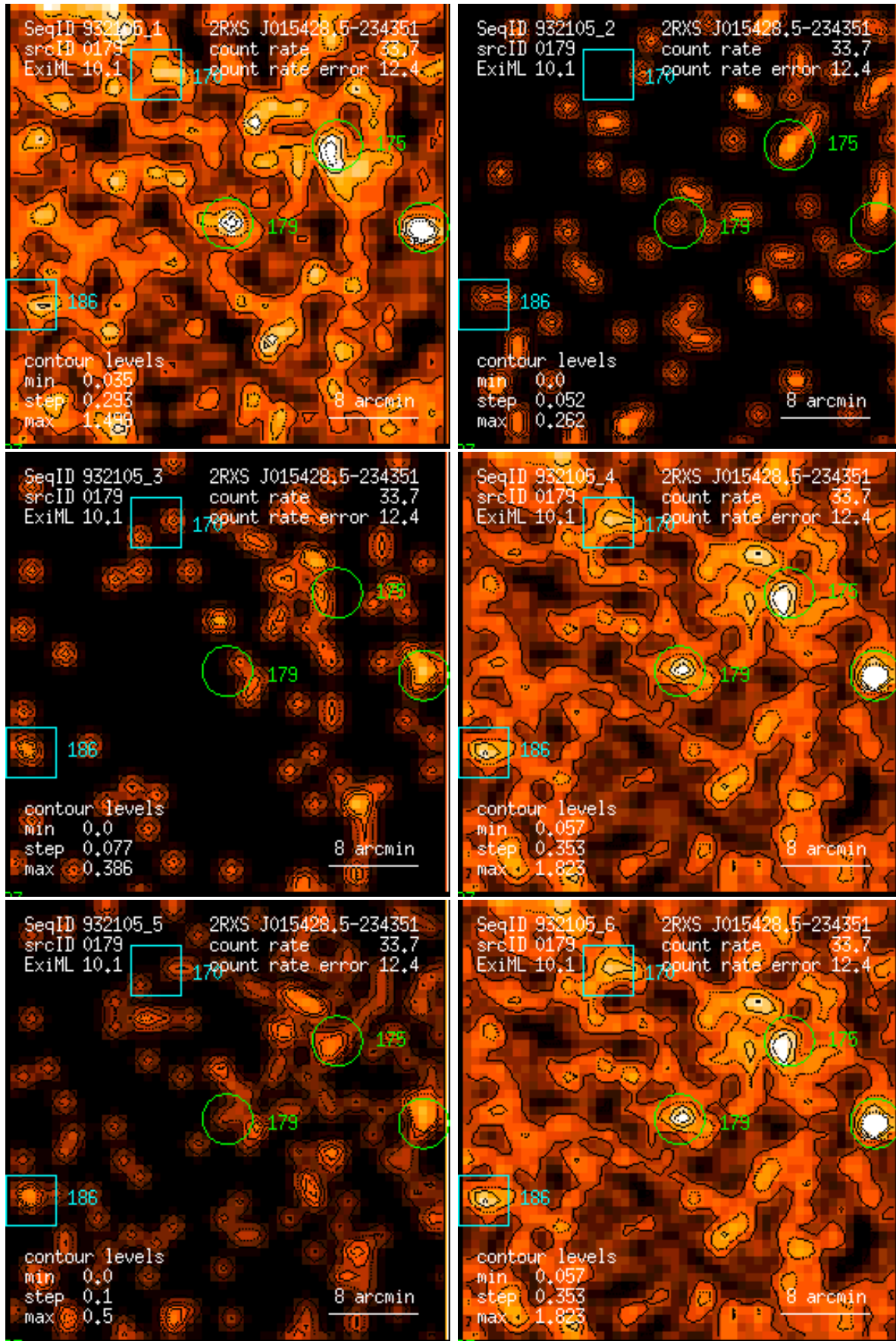
Figure 179: RASS 932105: detection 0179: band rate images, Gaussian filter: (1) PSPC channels 11 – 41, (2) 52 – 90, (3) 91 – 201, (4) 11 – 235, (5) 52 – 201, (6) 11 – 201. Broad band rates in counts/ks. Band rate contour levels in counts/ks/arcmin 2 .
