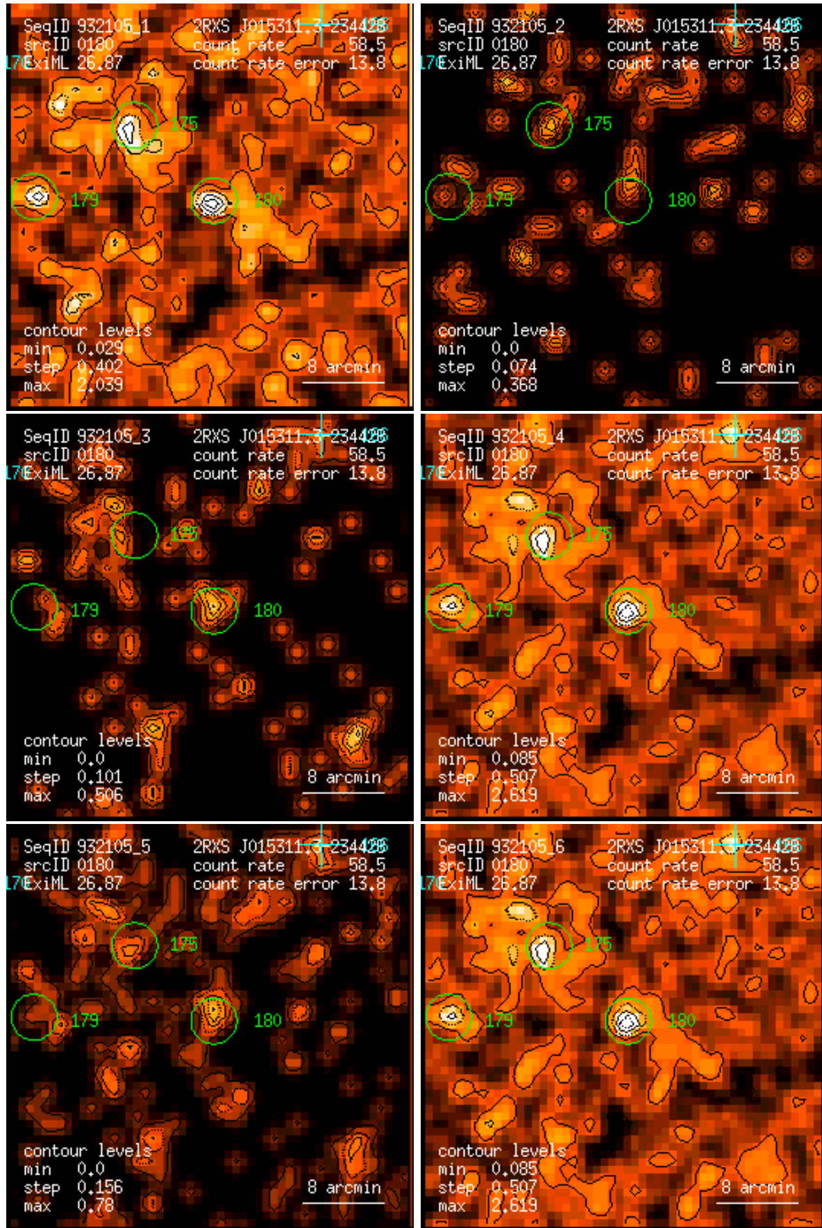
Figure 180: RASS 932105: detection 0180: band rate images, Gaussian filter: (1) PSPC channels 11 – 41, (2) 52 – 90, (3) 91 – 201, (4) 11 – 235, (5) 52 – 201, (6) 11 – 201. Broad band rates in counts/ks. Band rate contour levels in counts/ks/arcmin 2 .
