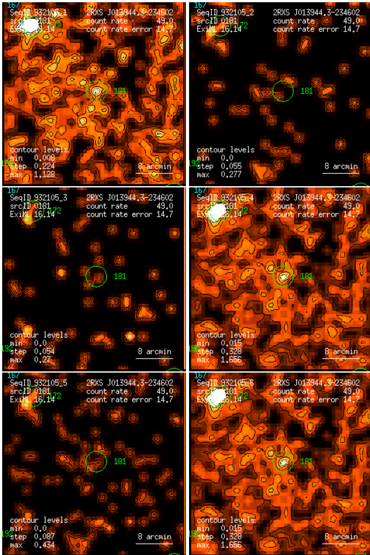
Figure 181: RASS 932105: detection 0181: band rate images, Gaussian filter: (1) PSPC channels 11 – 41, (2) 52 – 90, (3) 91 – 201, (4) 11 – 235, (5) 52 – 201, (6) 11 – 201. Broad band rates in counts/ks. Band rate contour levels in counts/ks/arcmin 2 .
