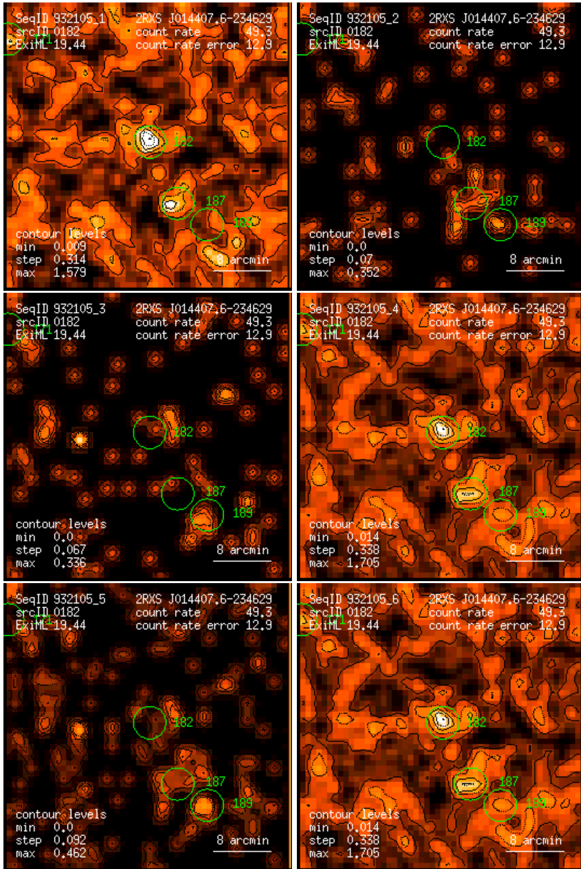
Figure 182: RASS 932105: detection 0182: band rate images, Gaussian filter: (1) PSPC channels 11 – 41, (2) 52 – 90, (3) 91 – 201, (4) 11 – 235, (5) 52 – 201, (6) 11 – 201. Broad band rates in counts/ks. Band rate contour levels in counts/ks/arcmin 2 .
