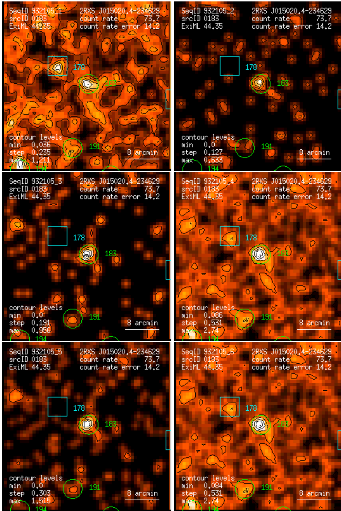
Figure 183: RASS 932105: detection 0183: band rate images, Gaussian filter: (1) PSPC channels 11 – 41, (2) 52 – 90, (3) 91 – 201, (4) 11 – 235, (5) 52 – 201, (6) 11 – 201. Broad band rates in counts/ks. Band rate contour levels in counts/ks/arcmin 2 .
