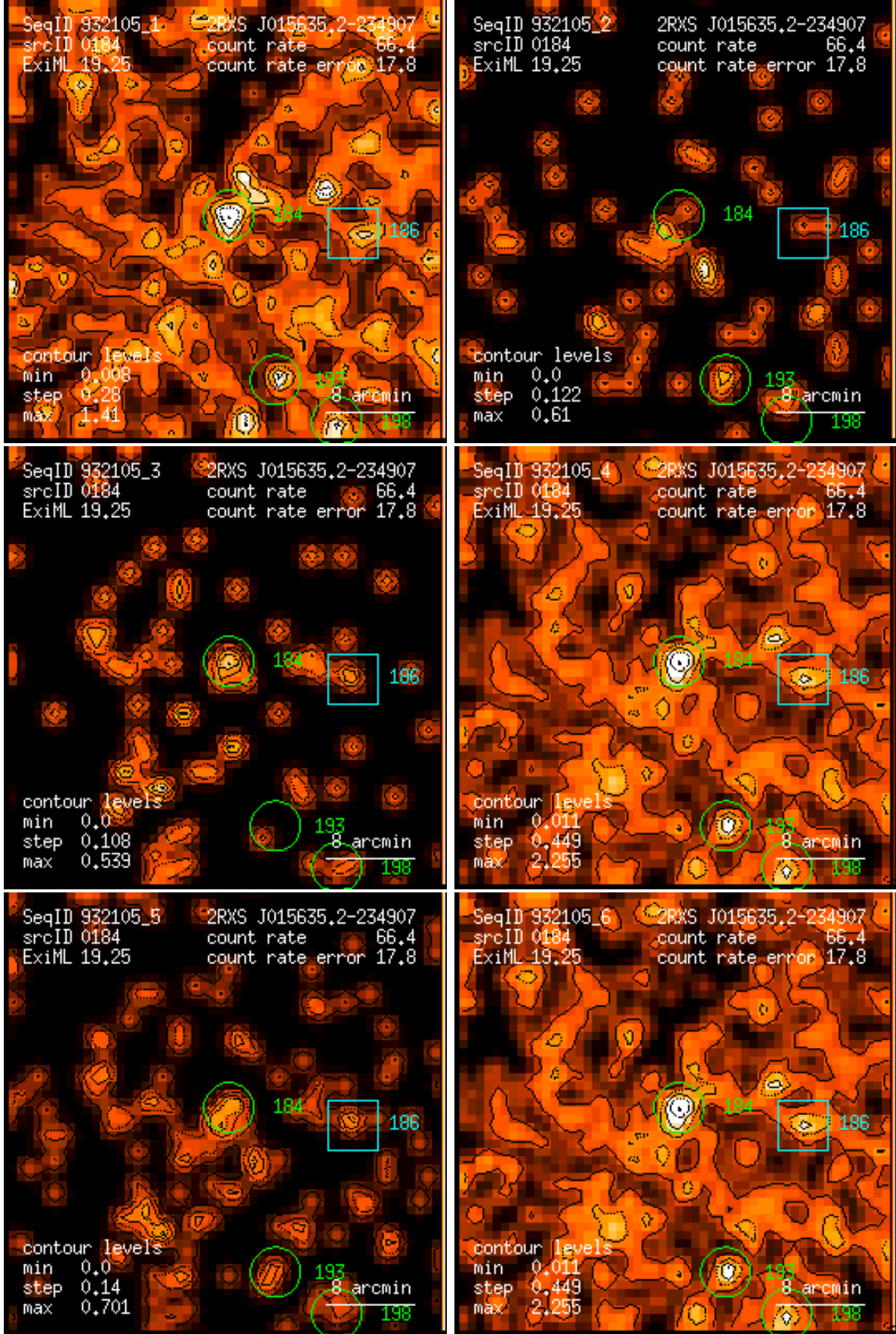
Figure 184: RASS 932105: detection 0184: band rate images, Gaussian filter: (1) PSPC channels 11 – 41, (2) 52 – 90, (3) 91 – 201, (4) 11 – 235, (5) 52 – 201, (6) 11 – 201. Broad band rates in counts/ks. Band rate contour levels in counts/ks/arcmin 2 .
