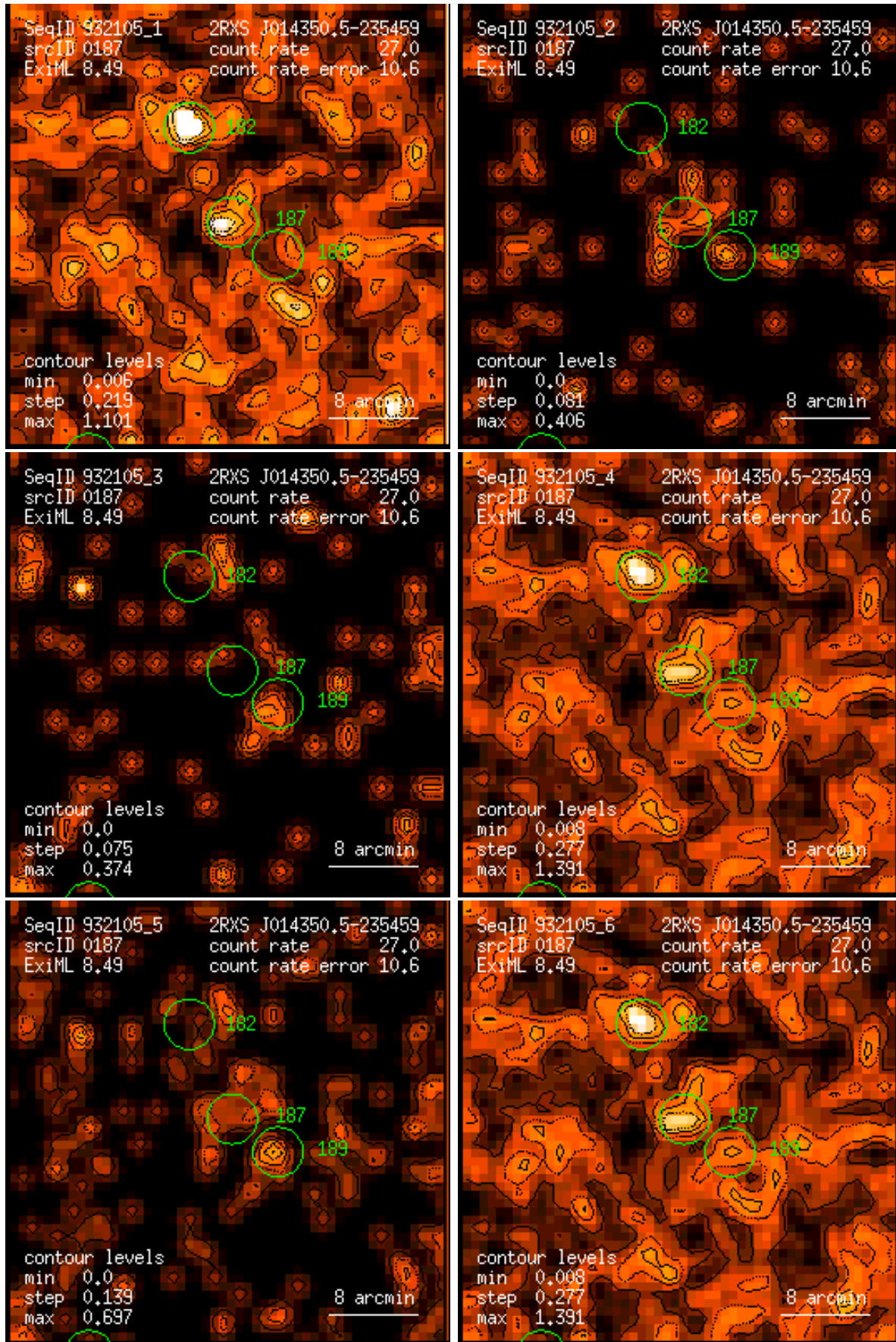
Figure 187: RASS 932105: detection 0187: band rate images, Gaussian filter: (1) PSPC channels 11 – 41, (2) 52 – 90, (3) 91 – 201, (4) 11 – 235, (5) 52 – 201, (6) 11 – 201. Broad band rates in counts/ks. Band rate contour levels in counts/ks/arcmin 2 .
