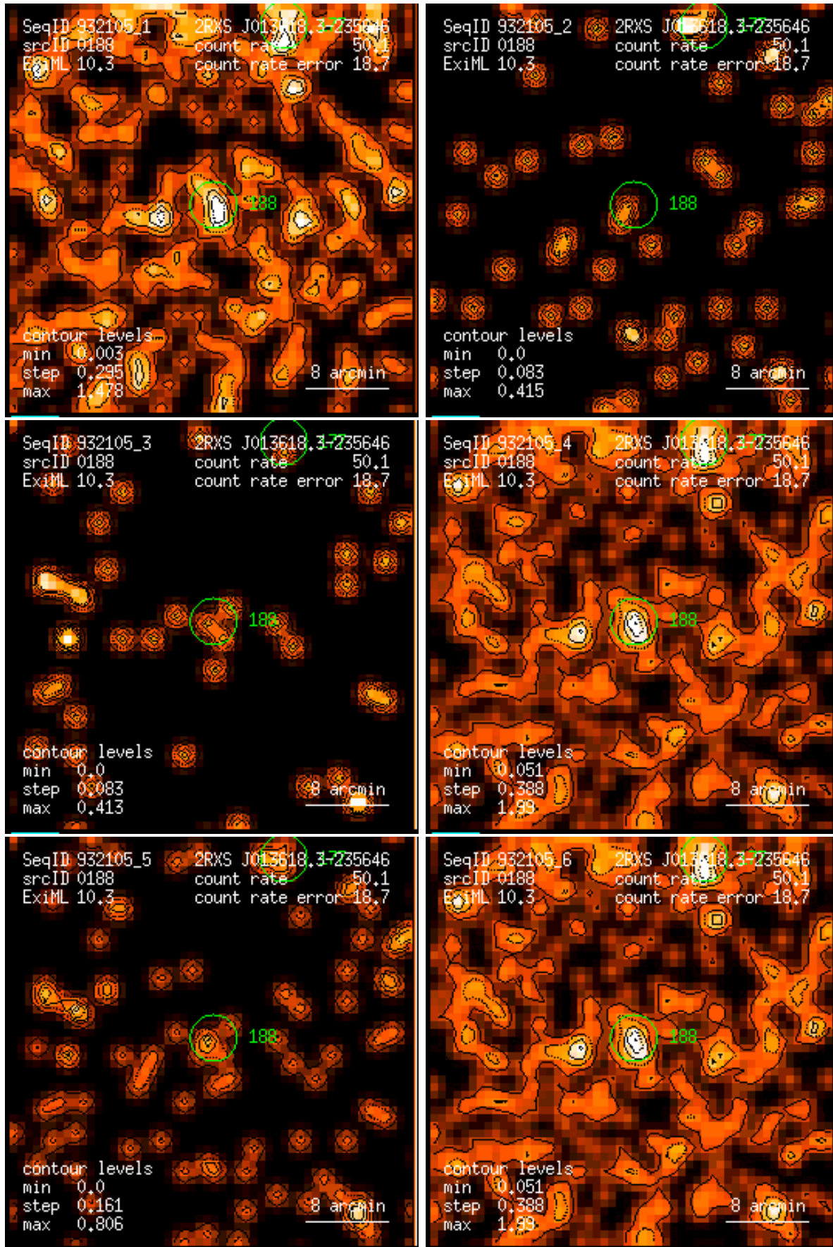
Figure 188: RASS 932105: detection 0188: band rate images, Gaussian filter: (1) PSPC channels 11 – 41, (2) 52 – 90, (3) 91 – 201, (4) 11 – 235, (5) 52 – 201, (6) 11 – 201. Broad band rates in counts/ks. Band rate contour levels in counts/ks/arcmin 2 .
