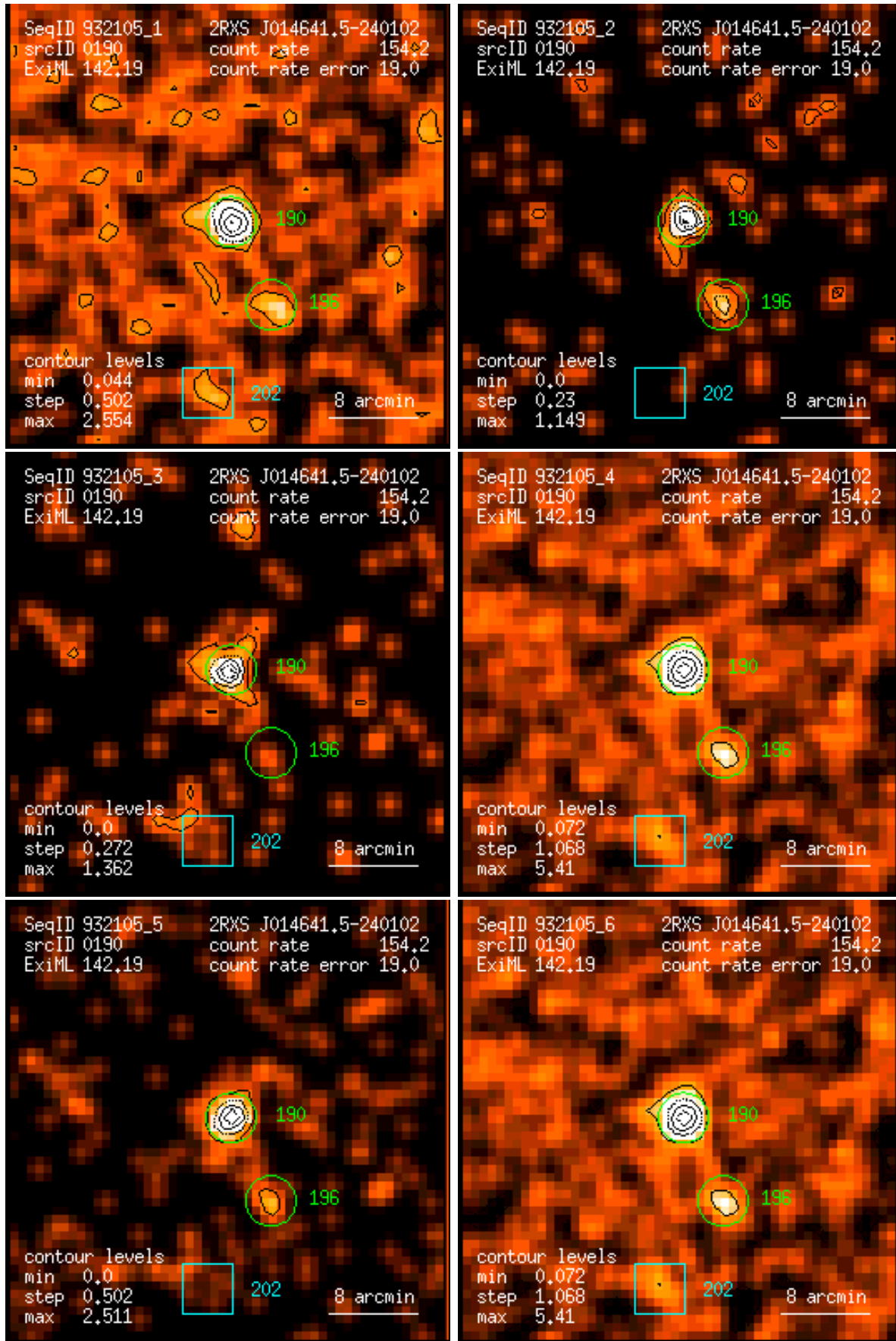
Figure 190: RASS 932105: detection 0190: band rate images, Gaussian filter: (1) PSPC channels 11 – 41, (2) 52 – 90, (3) 91 – 201, (4) 11 – 235, (5) 52 – 201, (6) 11 – 201. Broad band rates in counts/ks. Band rate contour levels in counts/ks/arcmin 2 .
