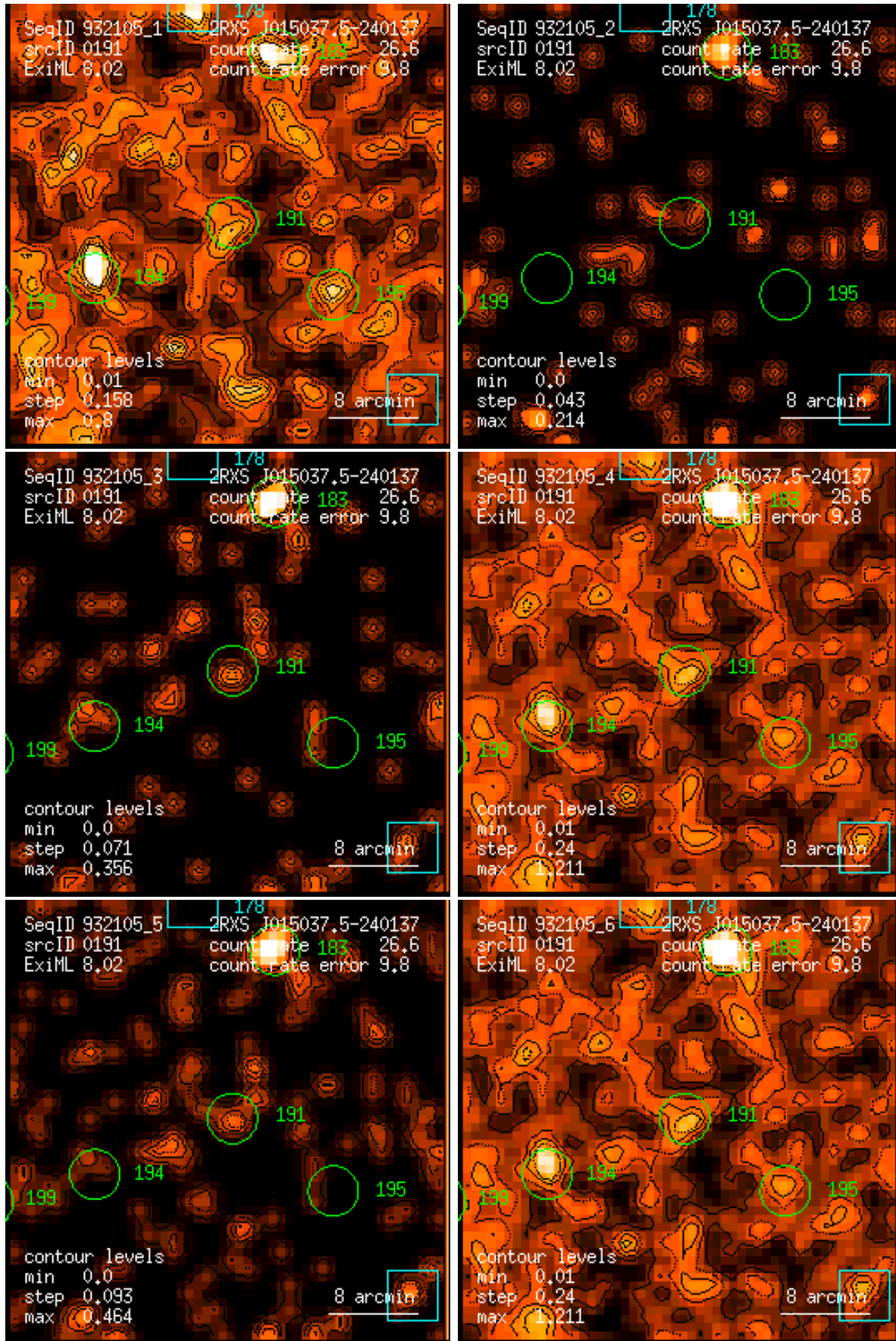
Figure 191: RASS 932105: detection 0191: band rate images, Gaussian filter: (1) PSPC channels 11 – 41, (2) 52 – 90, (3) 91 – 201, (4) 11 – 235, (5) 52 – 201, (6) 11 – 201. Broad band rates in counts/ks. Band rate contour levels in counts/ks/arcmin 2 .
