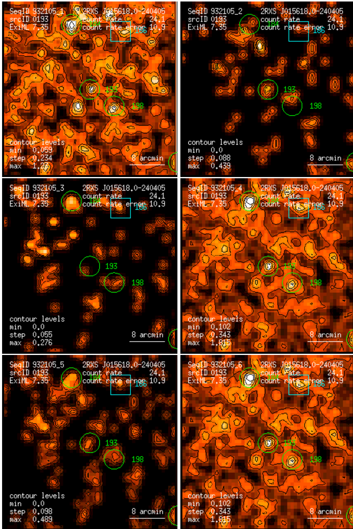
Figure 193: RASS 932105: detection 0193: band rate images, Gaussian filter: (1) PSPC channels 11 – 41, (2) 52 – 90, (3) 91 – 201, (4) 11 – 235, (5) 52 – 201, (6) 11 – 201. Broad band rates in counts/ks. Band rate contour levels in counts/ks/arcmin 2 .
