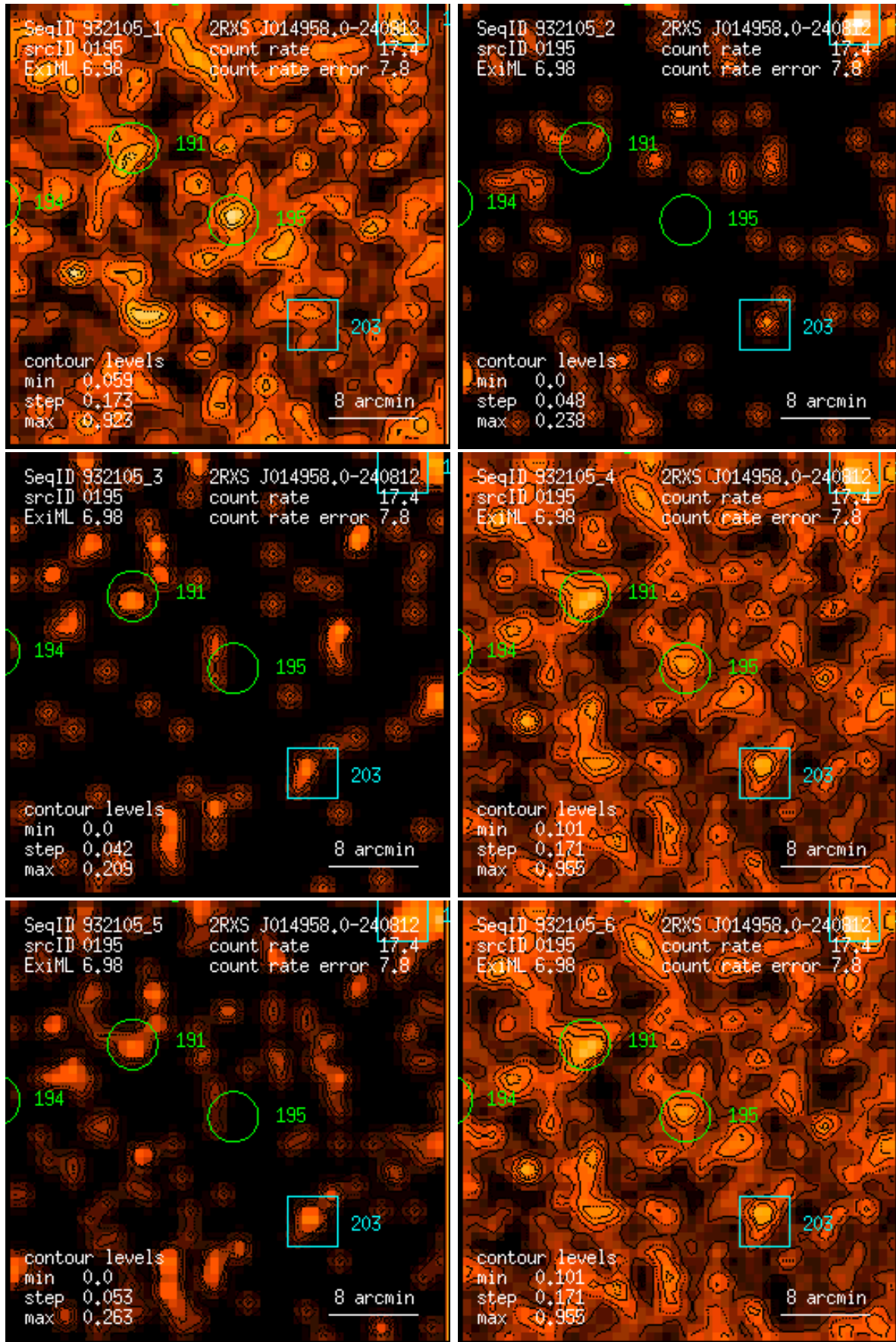
Figure 195: RASS 932105: detection 0195: band rate images, Gaussian filter: (1) PSPC channels 11 – 41, (2) 52 – 90, (3) 91 – 201, (4) 11 – 235, (5) 52 – 201, (6) 11 – 201. Broad band rates in counts/ks. Band rate contour levels in counts/ks/arcmin 2 .
