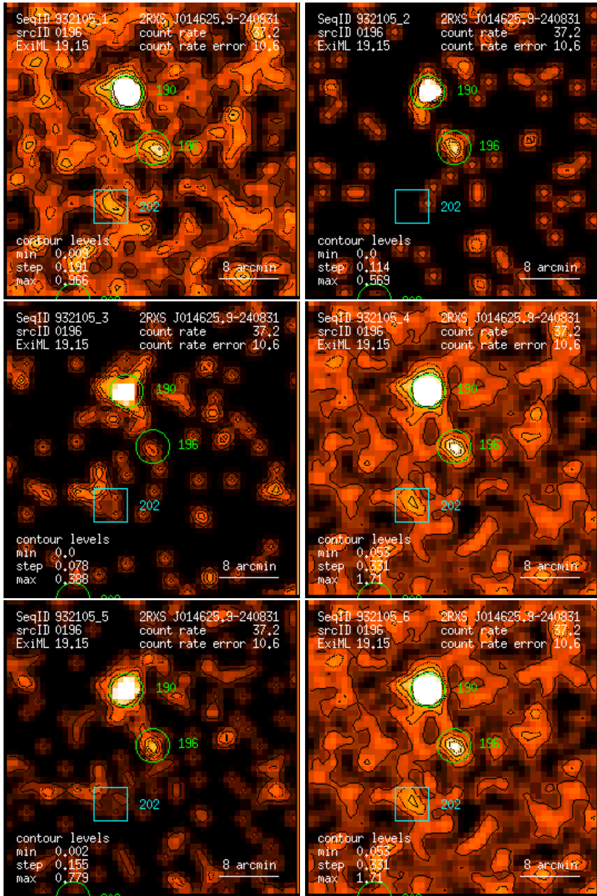
Figure 196: RASS 932105: detection 0196: band rate images, Gaussian filter: (1) PSPC channels 11 – 41, (2) 52 – 90, (3) 91 – 201, (4) 11 – 235, (5) 52 – 201, (6) 11 – 201. Broad band rates in counts/ks. Band rate contour levels in counts/ks/arcmin 2 .
