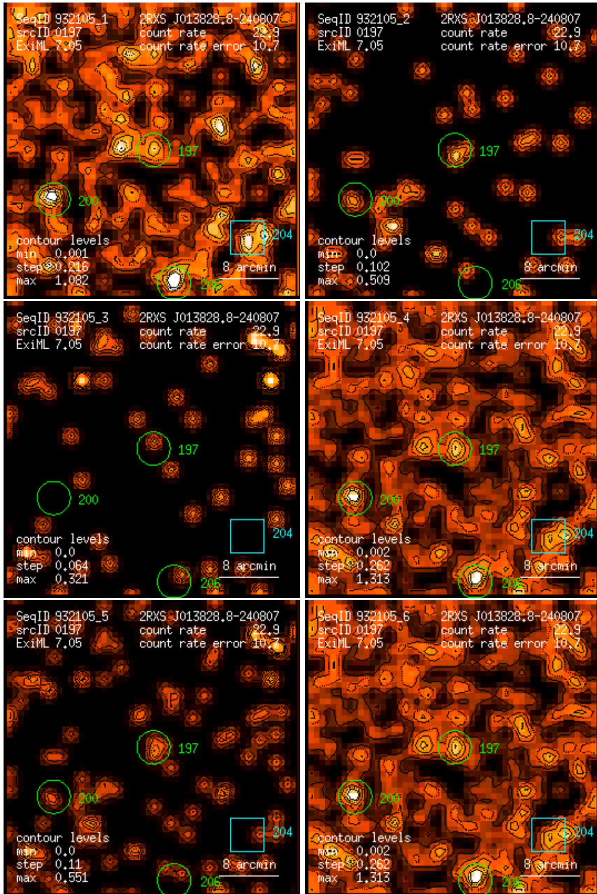
Figure 197: RASS 932105: detection 0197: band rate images, Gaussian filter: (1) PSPC channels 11 – 41, (2) 52 – 90, (3) 91 – 201, (4) 11 – 235, (5) 52 – 201, (6) 11 – 201. Broad band rates in counts/ks. Band rate contour levels in counts/ks/arcmin 2 .
