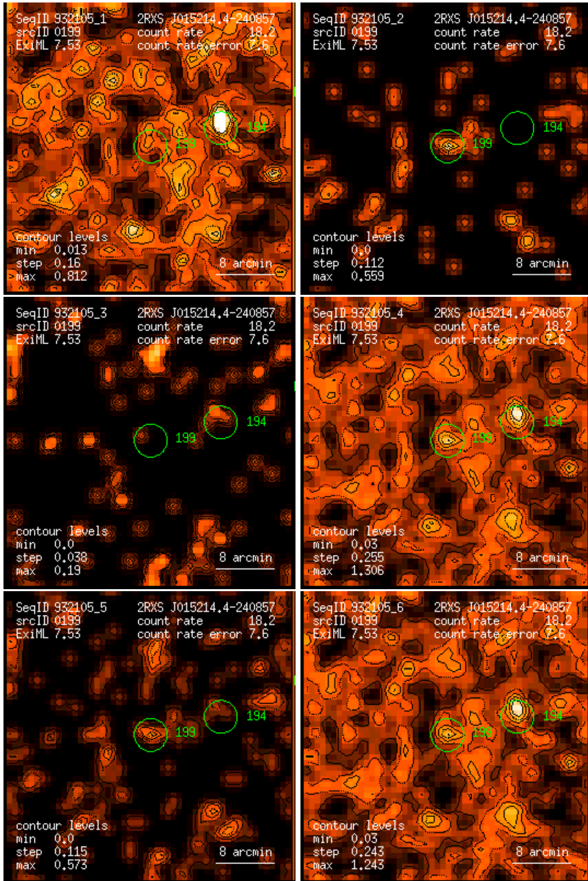
Figure 199: RASS 932105: detection 0199: band rate images, Gaussian filter: (1) PSPC channels 11 – 41, (2) 52 – 90, (3) 91 – 201, (4) 11 – 235, (5) 52 – 201, (6) 11 – 201. Broad band rates in counts/ks. Band rate contour levels in counts/ks/arcmin 2 .
