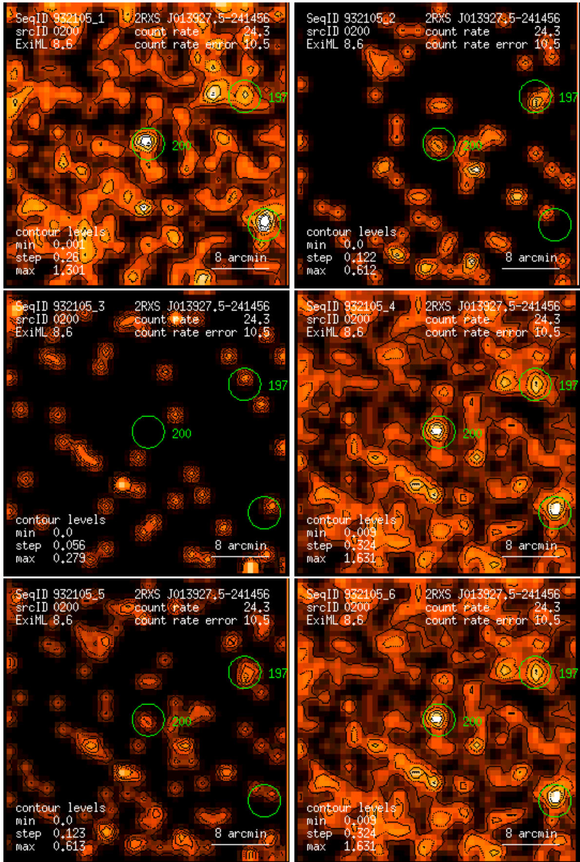
Figure 200: RASS 932105: detection 0200: band rate images, Gaussian filter: (1) PSPC channels 11 – 41, (2) 52 – 90, (3) 91 – 201, (4) 11 – 235, (5) 52 – 201, (6) 11 – 201. Broad band rates in counts/ks. Band rate contour levels in counts/ks/arcmin 2 .
