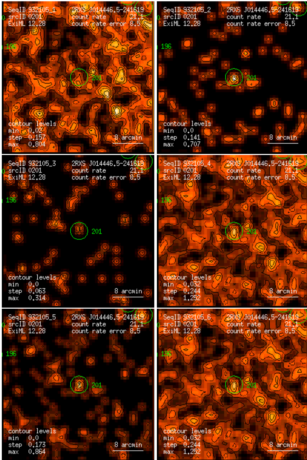
Figure 201: RASS 932105: detection 0201: band rate images, Gaussian filter: (1) PSPC channels 11 – 41, (2) 52 – 90, (3) 91 – 201, (4) 11 – 235, (5) 52 – 201, (6) 11 – 201. Broad band rates in counts/ks. Band rate contour levels in counts/ks/arcmin 2 .
