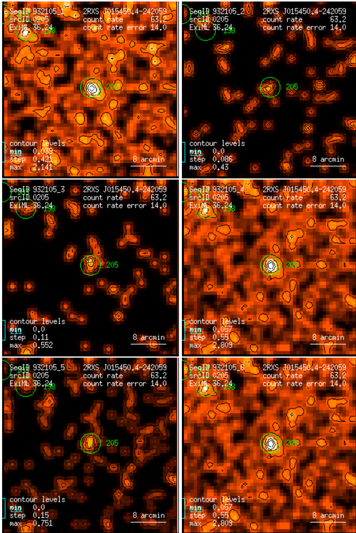
Figure 205: RASS 932105: detection 0205: band rate images, Gaussian filter: (1) PSPC channels 11 – 41, (2) 52 – 90, (3) 91 – 201, (4) 11 – 235, (5) 52 – 201, (6) 11 – 201. Broad band rates in counts/ks. Band rate contour levels in counts/ks/arcmin 2 .
