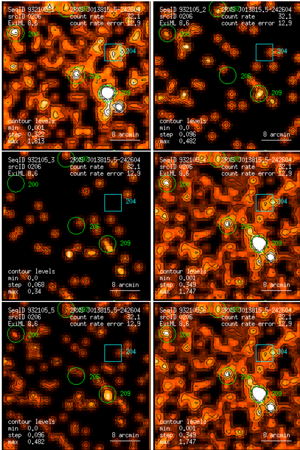
Figure 206: RASS 932105: detection 0206: band rate images, Gaussian filter: (1) PSPC channels 11 – 41, (2) 52 – 90, (3) 91 – 201, (4) 11 – 235, (5) 52 – 201, (6) 11 – 201. Broad band rates in counts/ks. Band rate contour levels in counts/ks/arcmin 2 .
