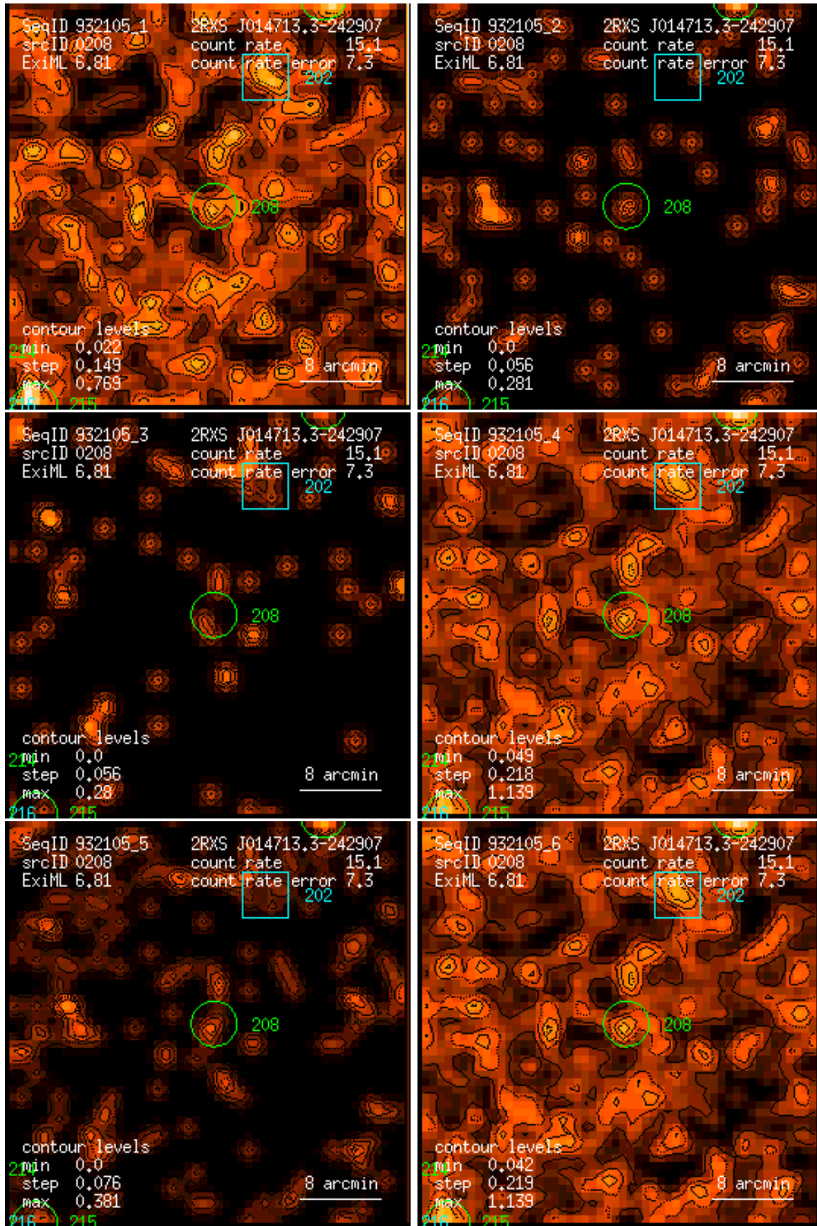
Figure 208: RASS 932105: detection 0208: band rate images, Gaussian filter: (1) PSPC channels 11 – 41, (2) 52 – 90, (3) 91 – 201, (4) 11 – 235, (5) 52 – 201, (6) 11 – 201. Broad band rates in counts/ks. Band rate contour levels in counts/ks/arcmin 2 .
