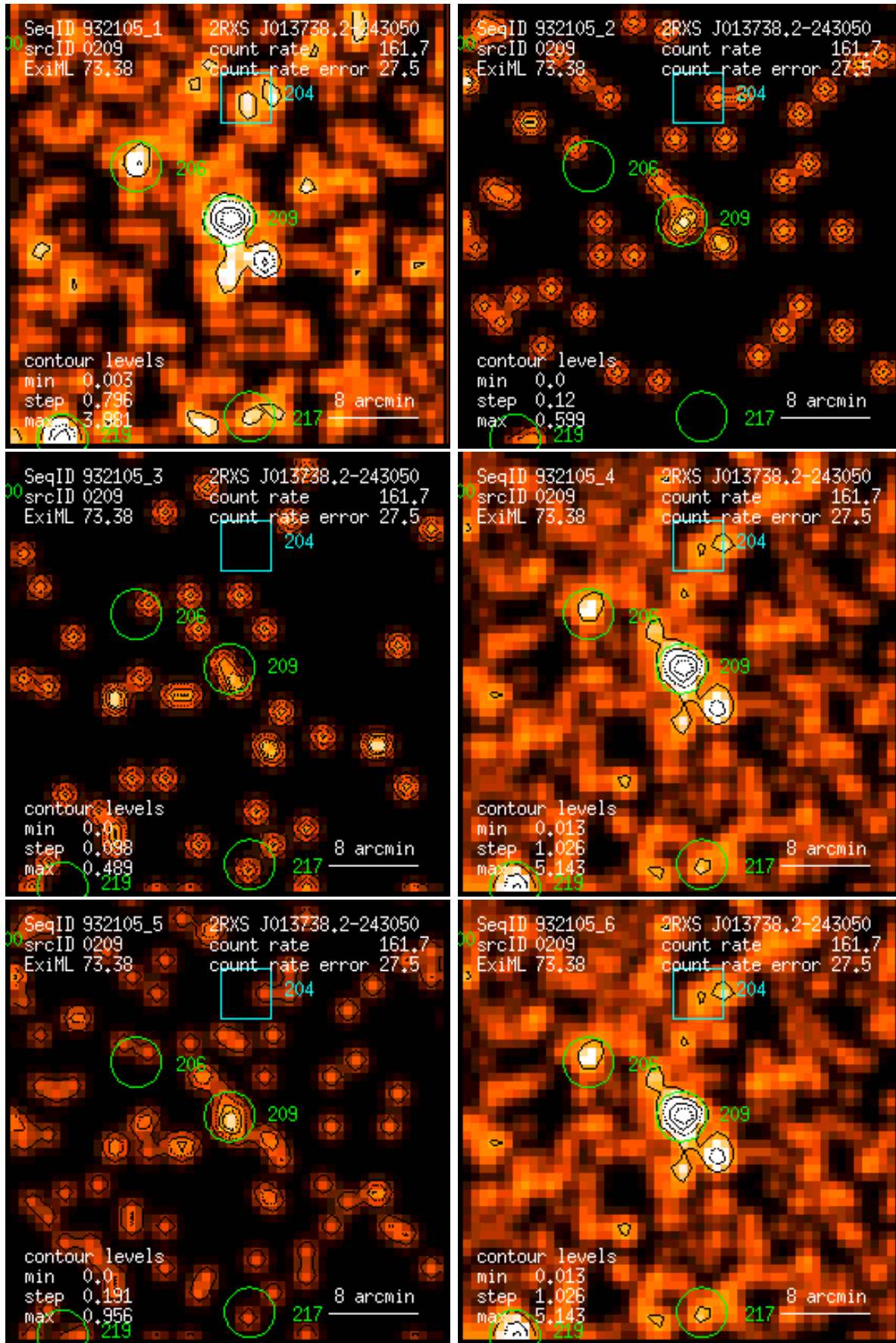
Figure 209: RASS 932105: detection 0209: band rate images, Gaussian filter: (1) PSPC channels 11 – 41, (2) 52 – 90, (3) 91 – 201, (4) 11 – 235, (5) 52 – 201, (6) 11 – 201. Broad band rates in counts/ks. Band rate contour levels in counts/ks/arcmin 2 .
