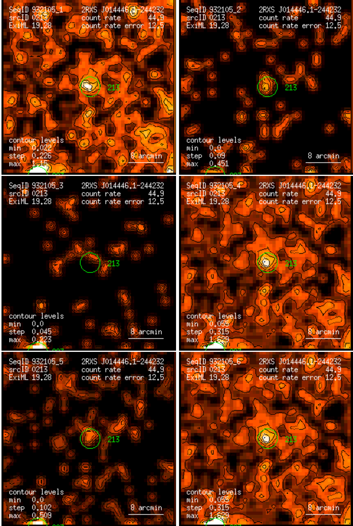
Figure 213: RASS 932105: detection 0213: band rate images, Gaussian filter: (1) PSPC channels 11 – 41, (2) 52 – 90, (3) 91 – 201, (4) 11 – 235, (5) 52 – 201, (6) 11 – 201. Broad band rates in counts/ks. Band rate contour levels in counts/ks/arcmin 2 .
