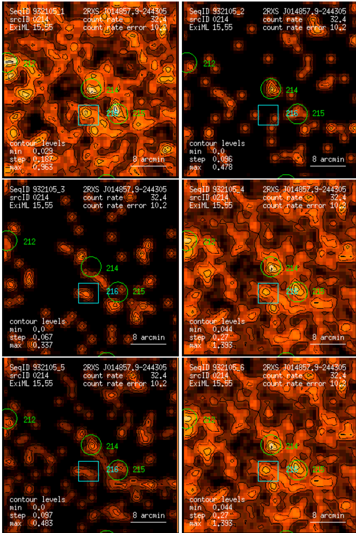
Figure 214: RASS 932105: detection 0214: band rate images, Gaussian filter: (1) PSPC channels 11 – 41, (2) 52 – 90, (3) 91 – 201, (4) 11 – 235, (5) 52 – 201, (6) 11 – 201. Broad band rates in counts/ks. Band rate contour levels in counts/ks/arcmin 2 .
