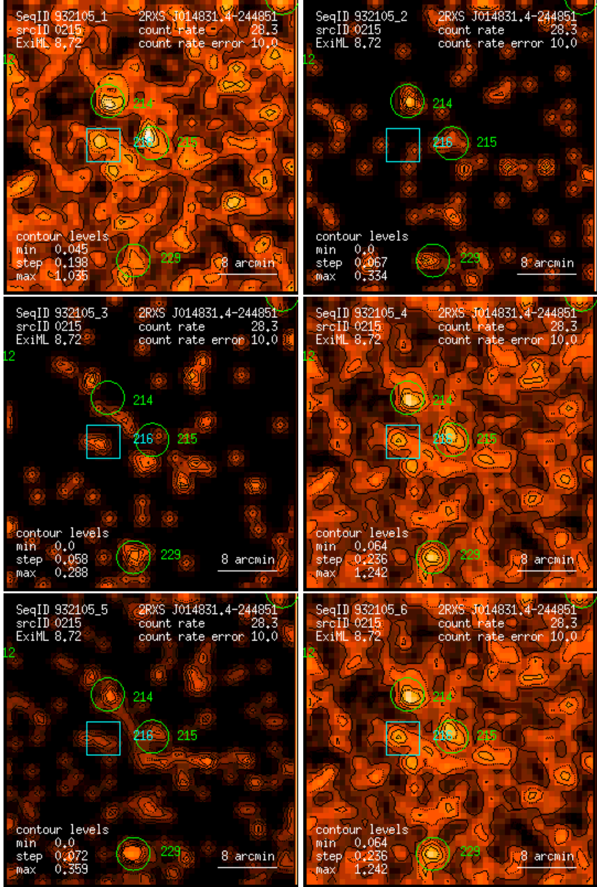
Figure 215: RASS 932105: detection 0215: band rate images, Gaussian filter: (1) PSPC channels 11 – 41, (2) 52 – 90, (3) 91 – 201, (4) 11 – 235, (5) 52 – 201, (6) 11 – 201. Broad band rates in counts/ks. Band rate contour levels in counts/ks/arcmin 2 .
