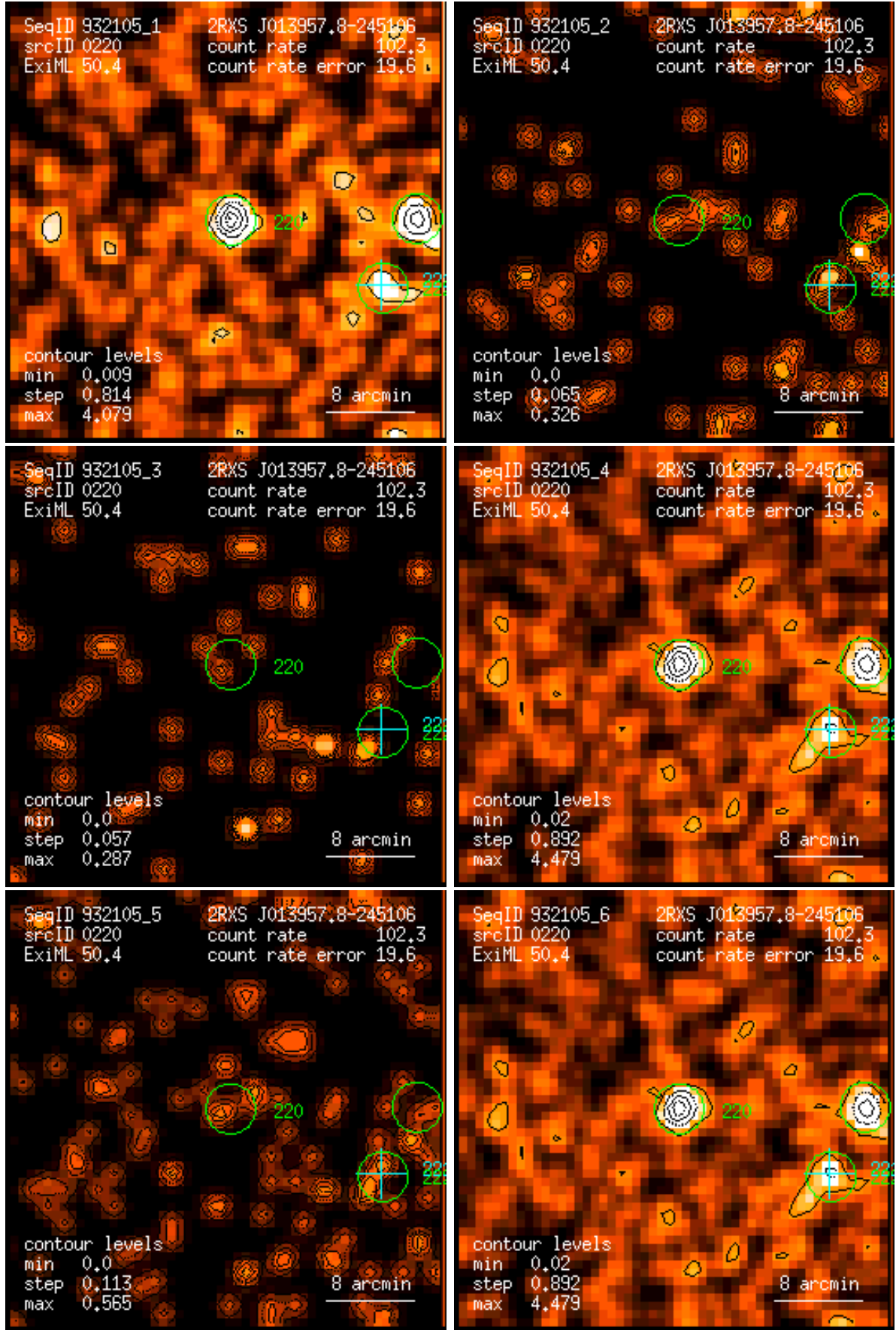
Figure 220: RASS 932105: detection 0220: band rate images, Gaussian filter: (1) PSPC channels 11 – 41, (2) 52 – 90, (3) 91 – 201, (4) 11 – 235, (5) 52 – 201, (6) 11 – 201. Broad band rates in counts/ks. Band rate contour levels in counts/ks/arcmin 2 .
