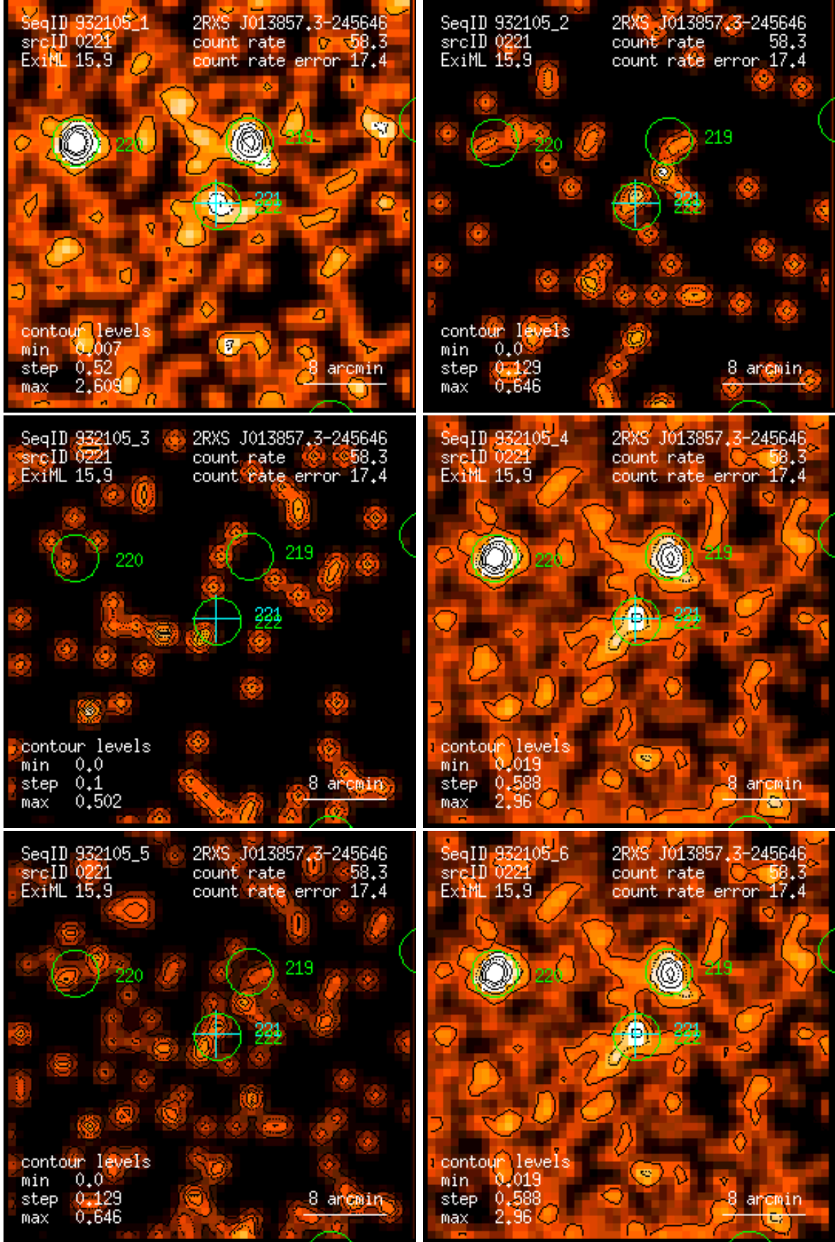
Figure 221: RASS 932105: detection 0221: band rate images, Gaussian filter: (1) PSPC channels 11 – 41, (2) 52 – 90, (3) 91 – 201, (4) 11 – 235, (5) 52 – 201, (6) 11 – 201. Broad band rates in counts/ks. Band rate contour levels in counts/ks/arcmin 2 .
